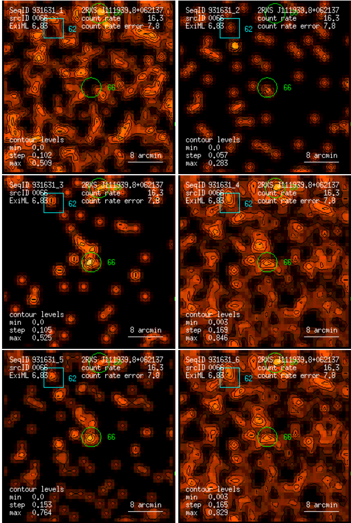
Figure 66: RASS 931631: detection 0066: band rate images, Gaussian filter: (1) PSPC channels 11 – 41, (2) 52 – 90, (3) 91 – 201, (4) 11 – 235, (5) 52 – 201, (6) 11 – 201. Broad band rates in counts/ks. Band rate contour levels in counts/ks/arcmin 2 .
