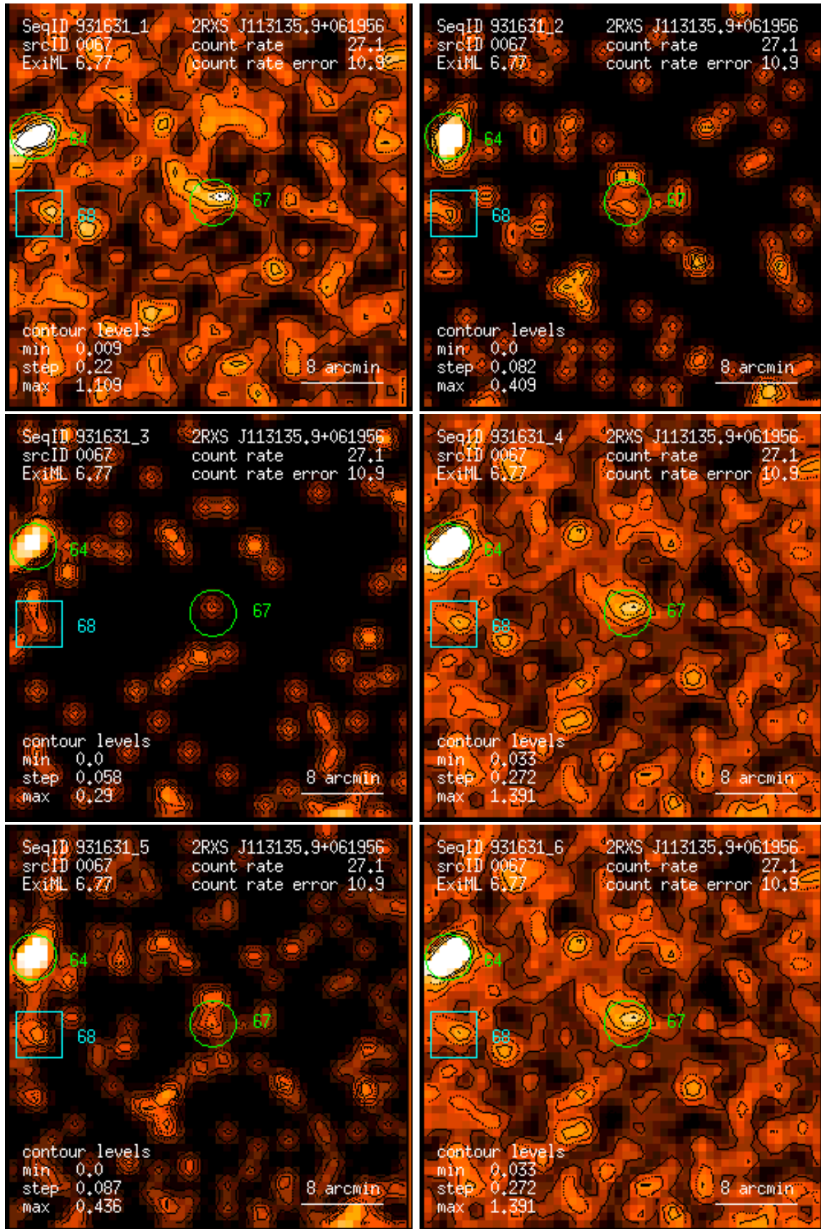
Figure 67: RASS 931631: detection 0067: band rate images, Gaussian filter: (1) PSPC channels 11 – 41, (2) 52 – 90, (3) 91 – 201, (4) 11 – 235, (5) 52 – 201, (6) 11 – 201. Broad band rates in counts/ks. Band rate contour levels in counts/ks/arcmin 2 .
