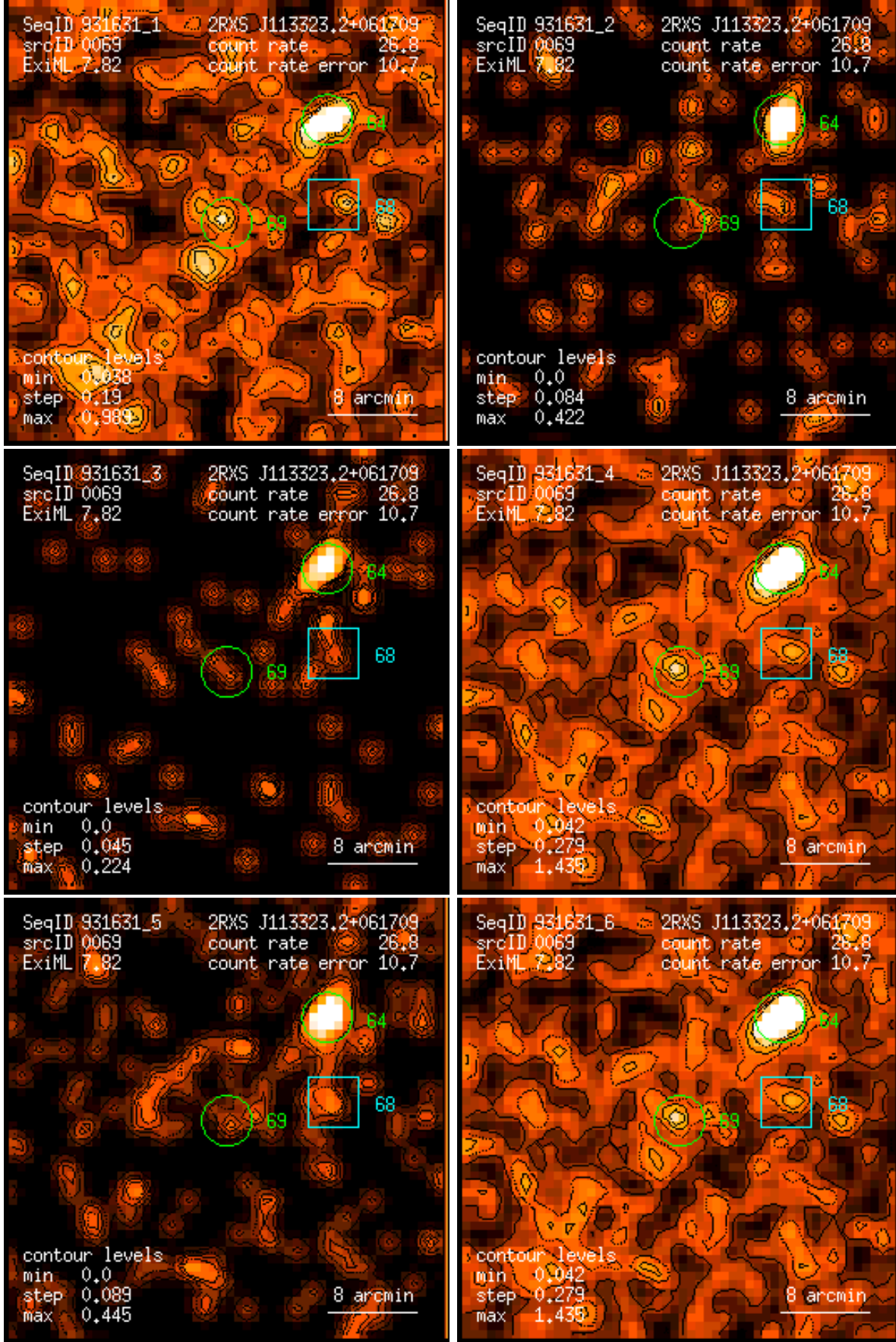
Figure 69: RASS 931631: detection 0069: band rate images, Gaussian filter: (1) PSPC channels 11 – 41, (2) 52 – 90, (3) 91 – 201, (4) 11 – 235, (5) 52 – 201, (6) 11 – 201. Broad band rates in counts/ks. Band rate contour levels in counts/ks/arcmin 2 .
