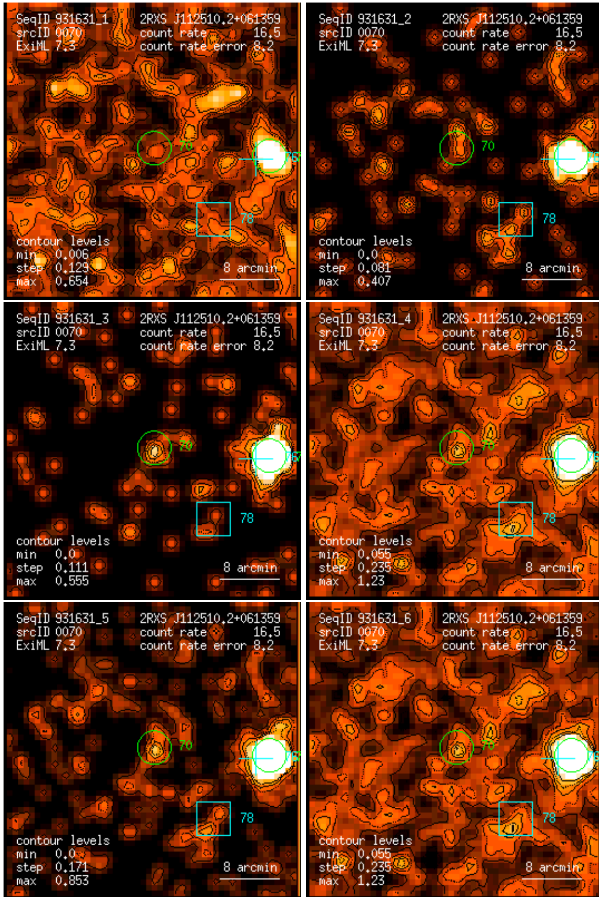
Figure 70: RASS 931631: detection 0070: band rate images, Gaussian filter: (1) PSPC channels 11 – 41, (2) 52 – 90, (3) 91 – 201, (4) 11 – 235, (5) 52 – 201, (6) 11 – 201. Broad band rates in counts/ks. Band rate contour levels in counts/ks/arcmin 2 .
