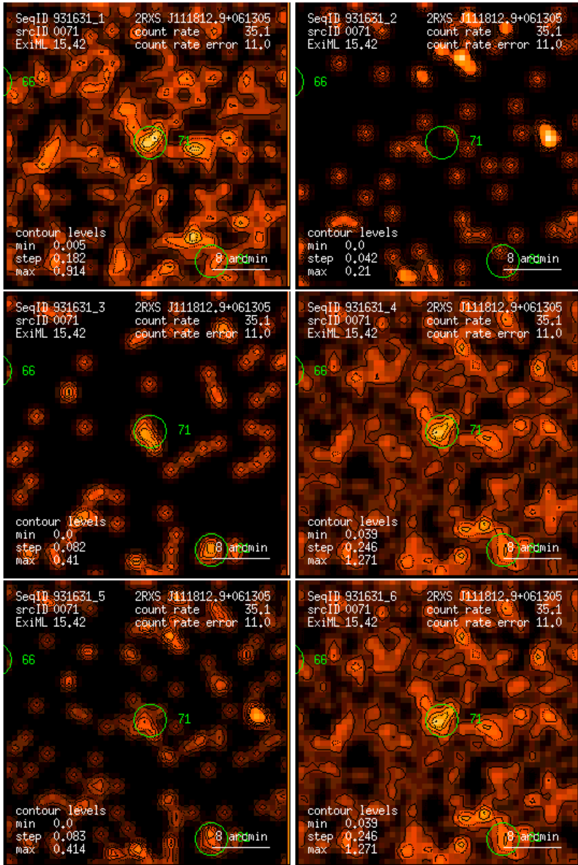
Figure 71: RASS 931631: detection 0071: band rate images, Gaussian filter: (1) PSPC channels 11 – 41, (2) 52 – 90, (3) 91 – 201, (4) 11 – 235, (5) 52 – 201, (6) 11 – 201. Broad band rates in counts/ks. Band rate contour levels in counts/ks/arcmin 2 .
