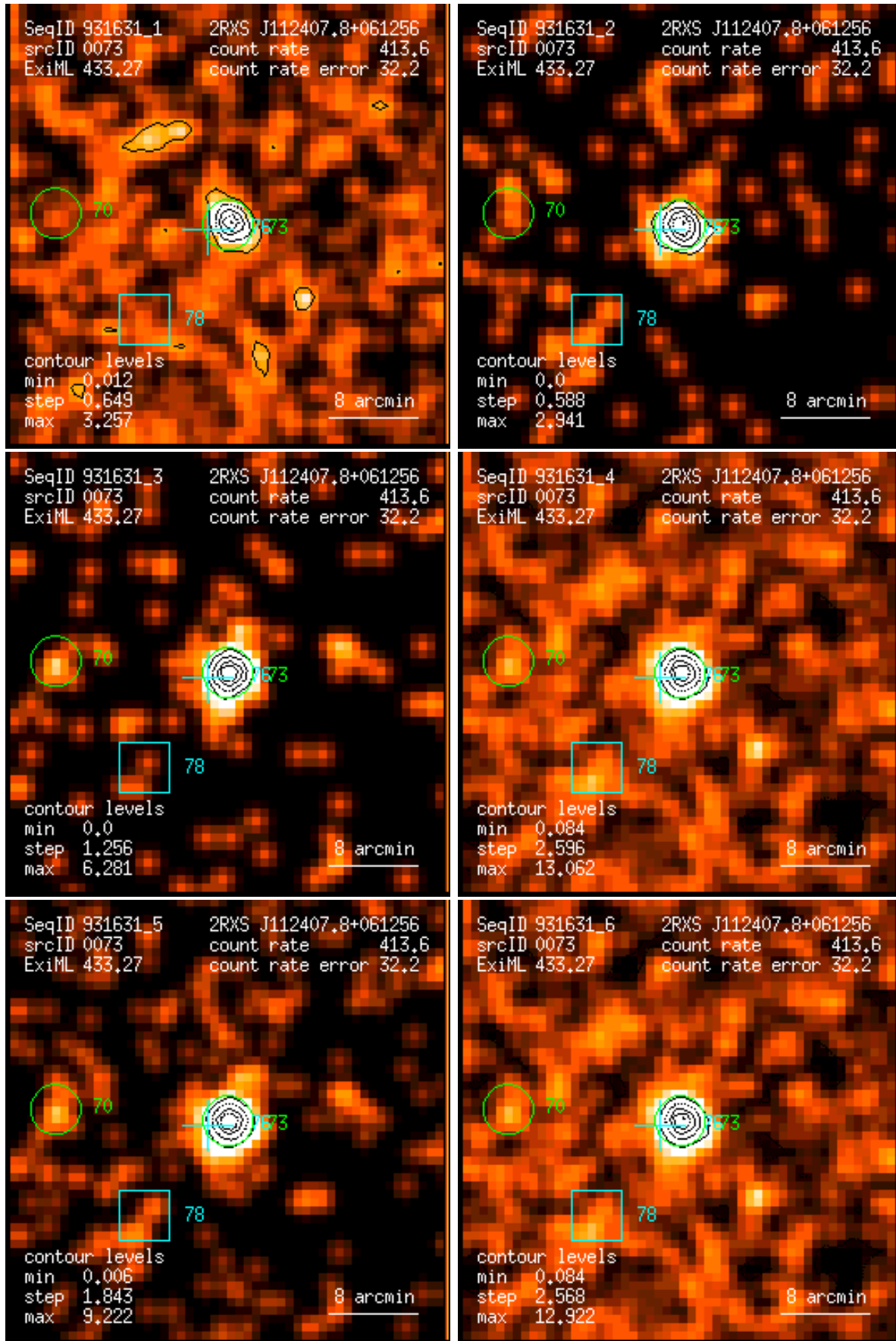
Figure 73: RASS 931631: detection 0073: band rate images, Gaussian filter: (1) PSPC channels 11 – 41, (2) 52 – 90, (3) 91 – 201, (4) 11 – 235, (5) 52 – 201, (6) 11 – 201. Broad band rates in counts/ks. Band rate contour levels in counts/ks/arcmin 2 .
