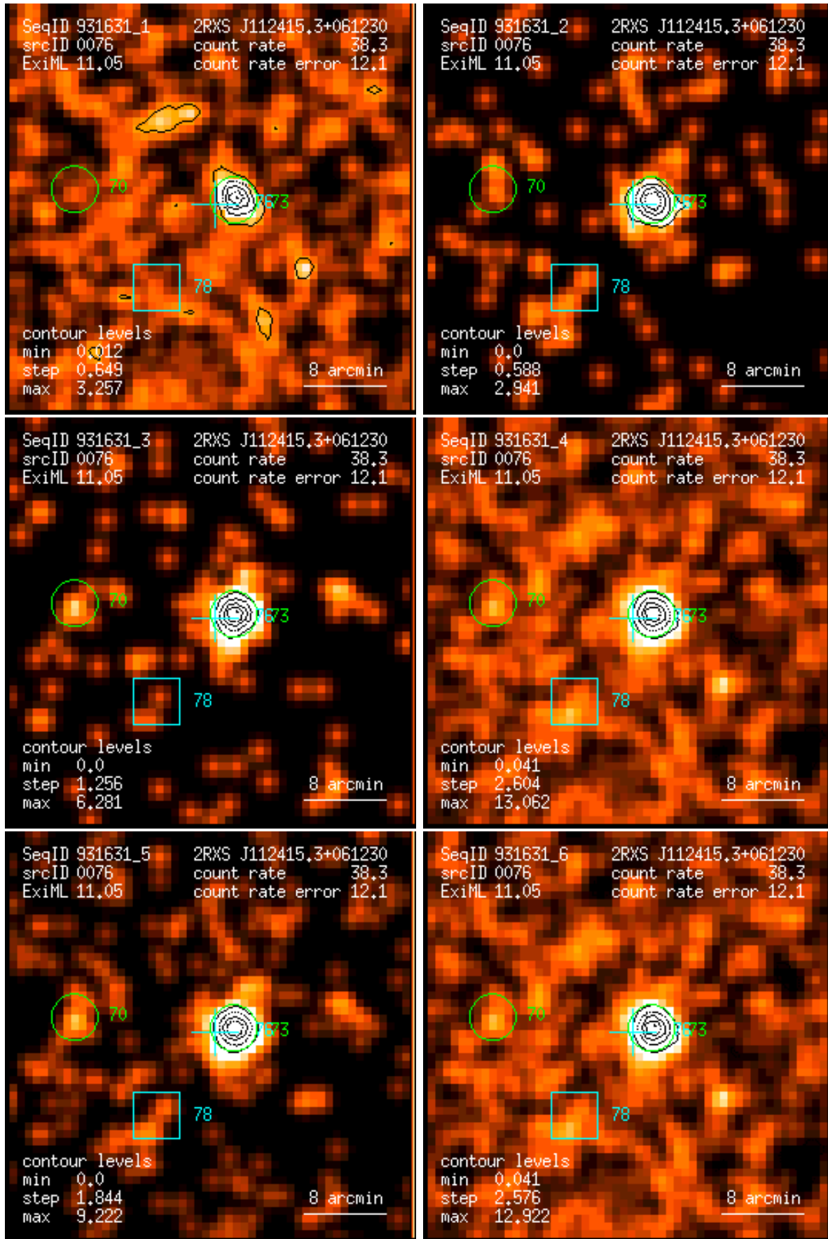
Figure 76: RASS 931631: detection 0076: band rate images, Gaussian filter: (1) PSPC channels 11 – 41, (2) 52 – 90, (3) 91 – 201, (4) 11 – 235, (5) 52 – 201, (6) 11 – 201. Broad band rates in counts/ks. Band rate contour levels in counts/ks/arcmin 2 .
