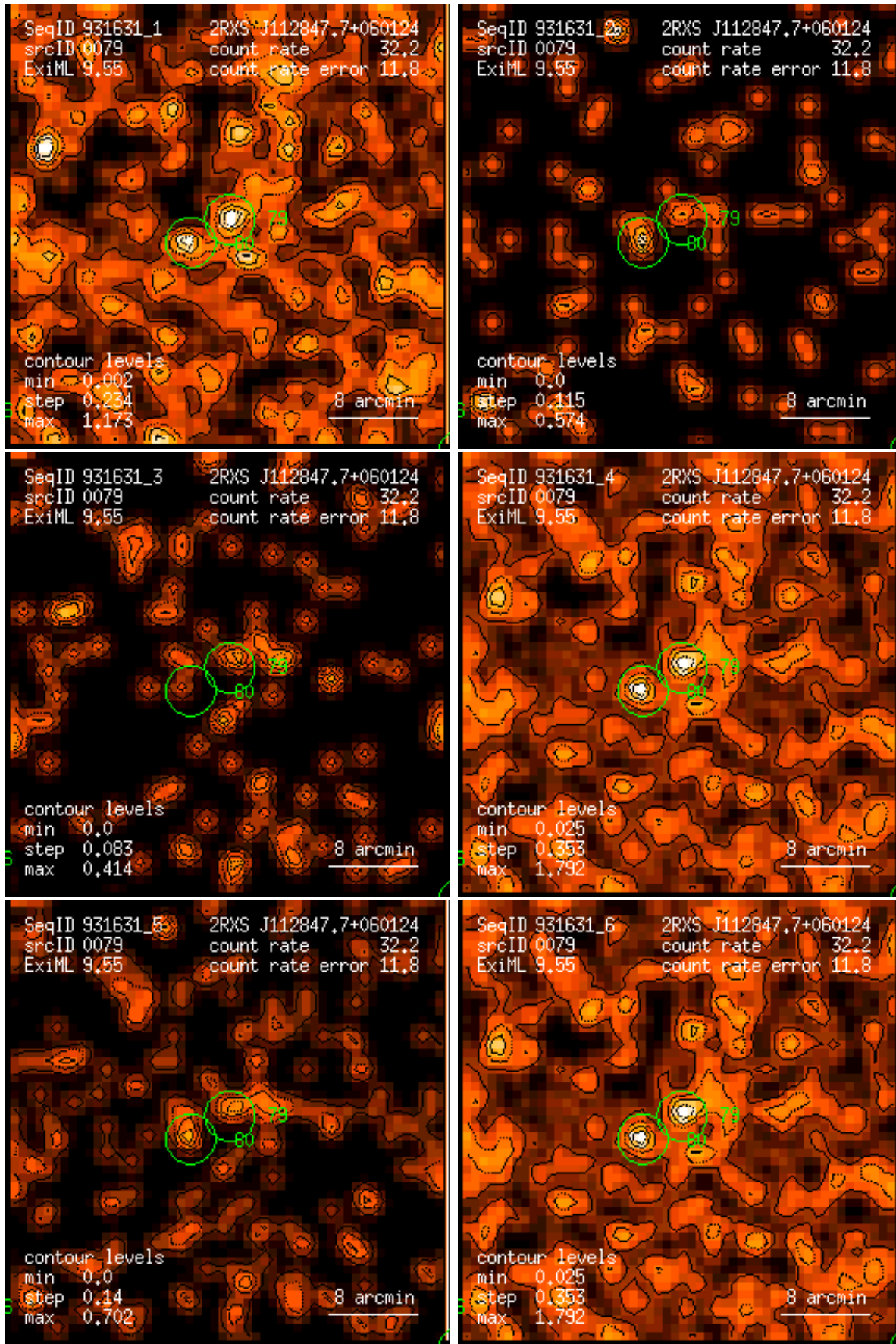
Figure 79: RASS 931631: detection 0079: band rate images, Gaussian filter: (1) PSPC channels 11 – 41, (2) 52 – 90, (3) 91 – 201, (4) 11 – 235, (5) 52 – 201, (6) 11 – 201. Broad band rates in counts/ks. Band rate contour levels in counts/ks/arcmin 2 .
