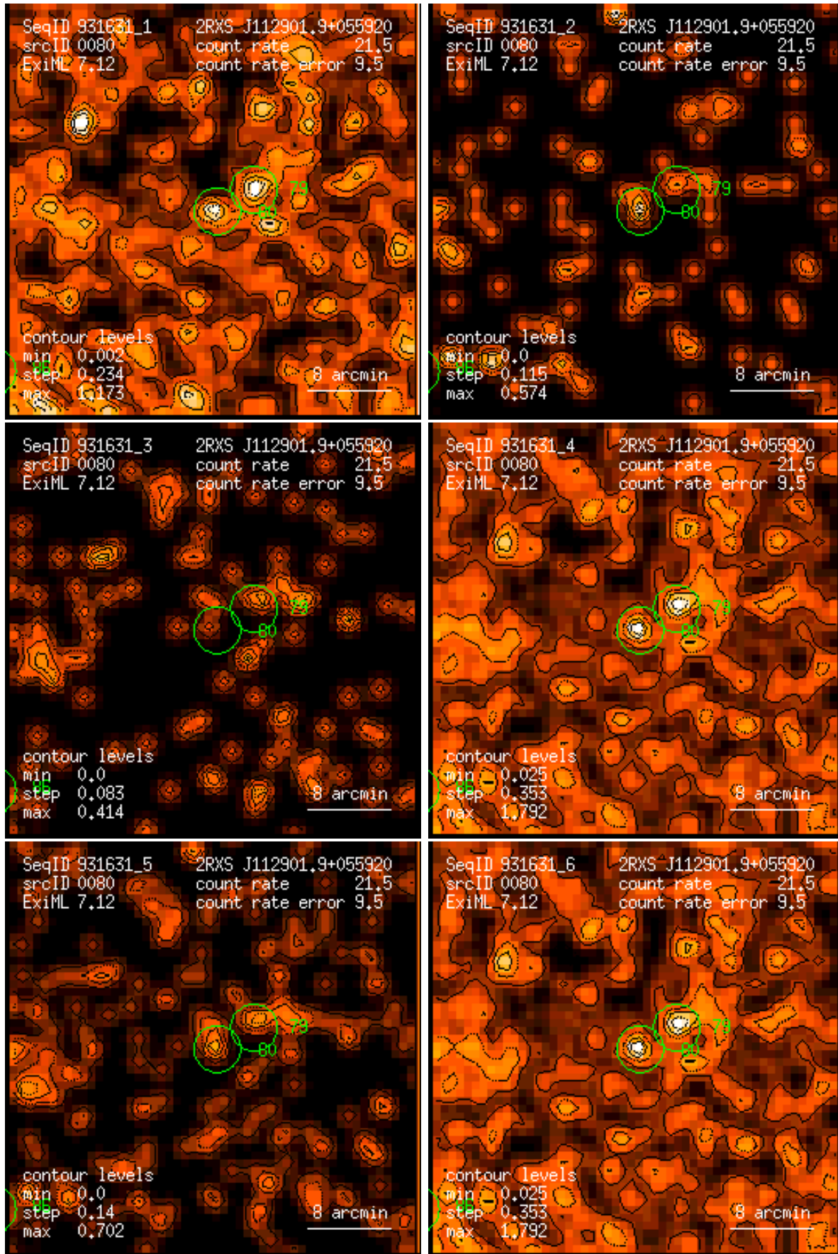
Figure 80: RASS 931631: detection 0080: band rate images, Gaussian filter: (1) PSPC channels 11 – 41, (2) 52 – 90, (3) 91 – 201, (4) 11 – 235, (5) 52 – 201, (6) 11 – 201. Broad band rates in counts/ks. Band rate contour levels in counts/ks/arcmin 2 .
