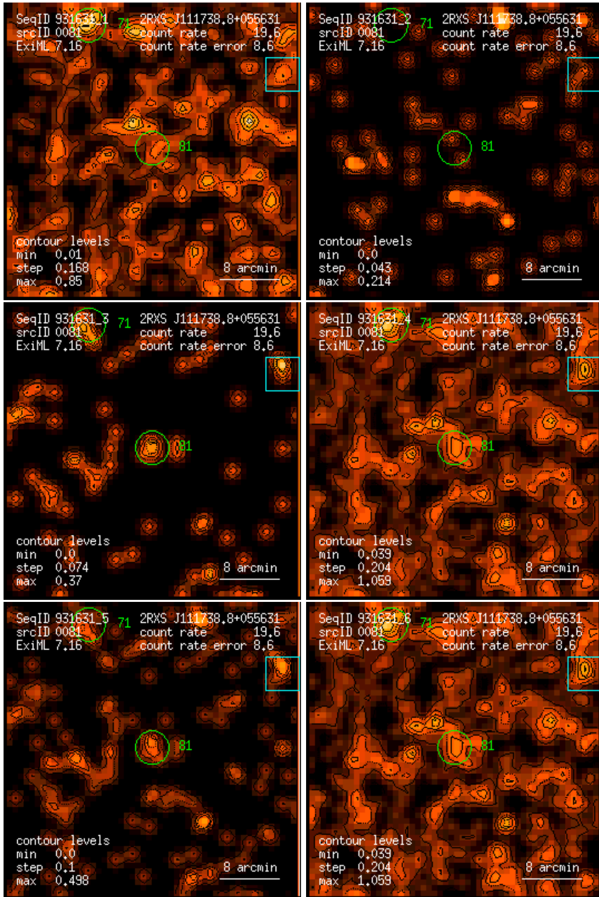
Figure 81: RASS 931631: detection 0081: band rate images, Gaussian filter: (1) PSPC channels 11 – 41, (2) 52 – 90, (3) 91 – 201, (4) 11 – 235, (5) 52 – 201, (6) 11 – 201. Broad band rates in counts/ks. Band rate contour levels in counts/ks/arcmin 2 .
