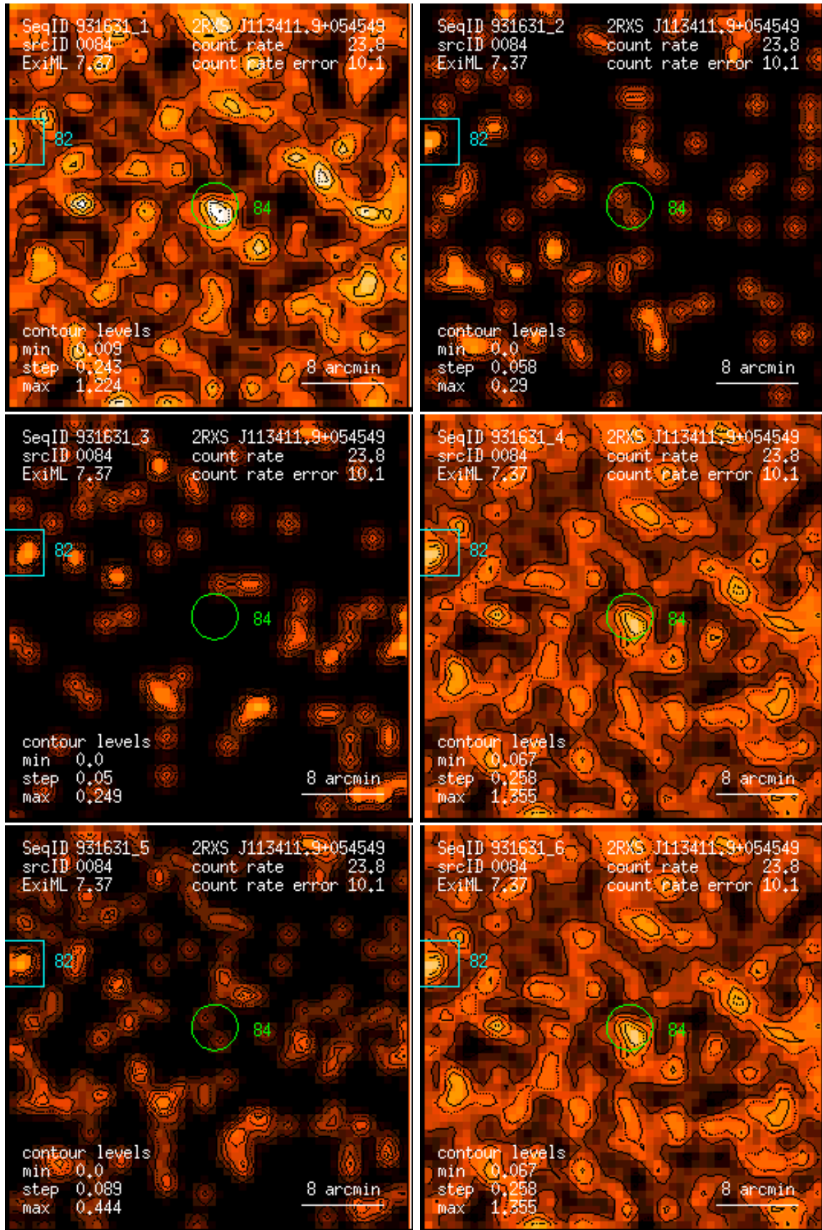
Figure 84: RASS 931631: detection 0084: band rate images, Gaussian filter: (1) PSPC channels 11 – 41, (2) 52 – 90, (3) 91 – 201, (4) 11 – 235, (5) 52 – 201, (6) 11 – 201. Broad band rates in counts/ks. Band rate contour levels in counts/ks/arcmin 2 .
