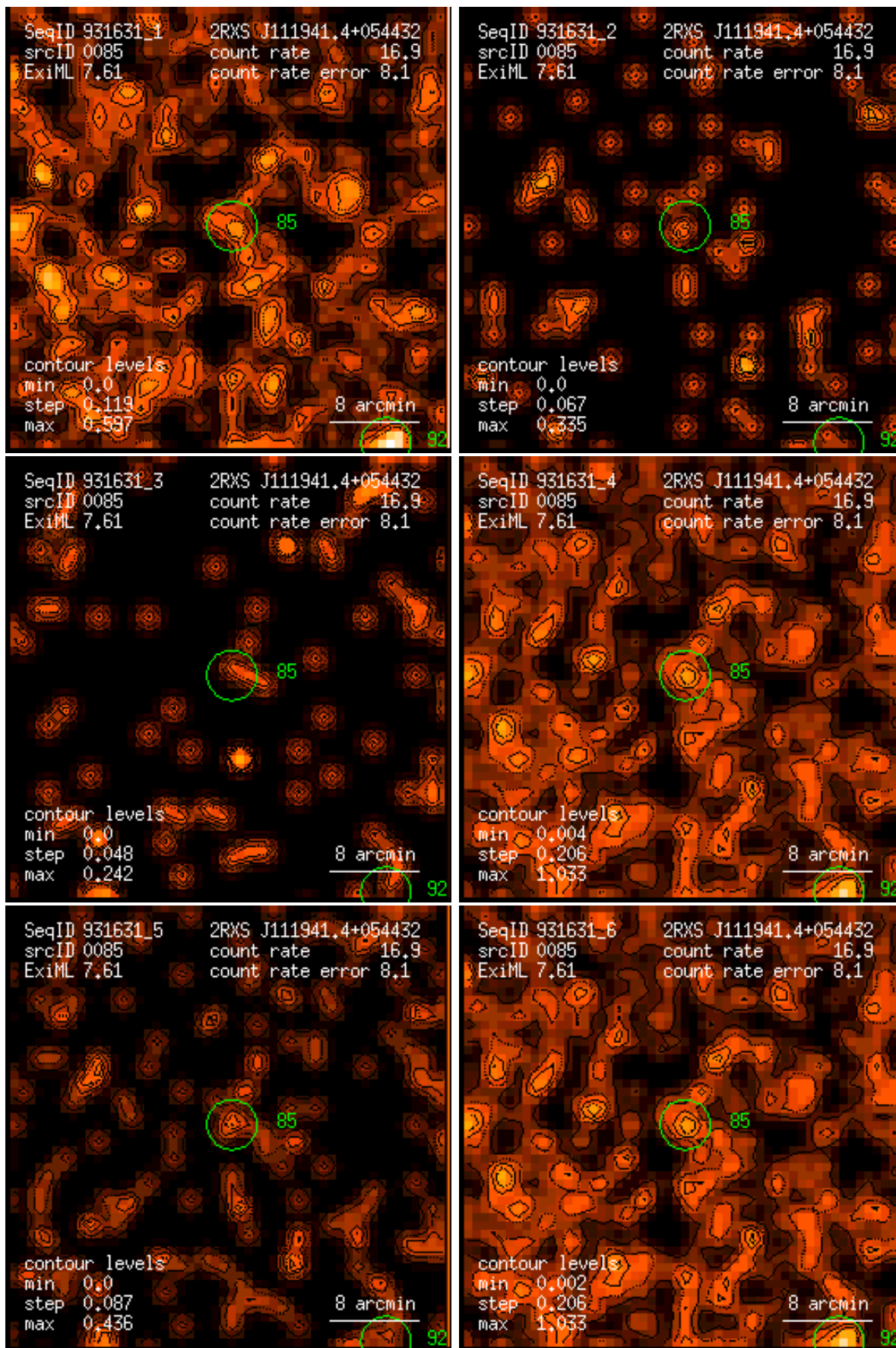
Figure 85: RASS 931631: detection 0085: band rate images, Gaussian filter: (1) PSPC channels 11 – 41, (2) 52 – 90, (3) 91 – 201, (4) 11 – 235, (5) 52 – 201, (6) 11 – 201. Broad band rates in counts/ks. Band rate contour levels in counts/ks/arcmin 2 .
