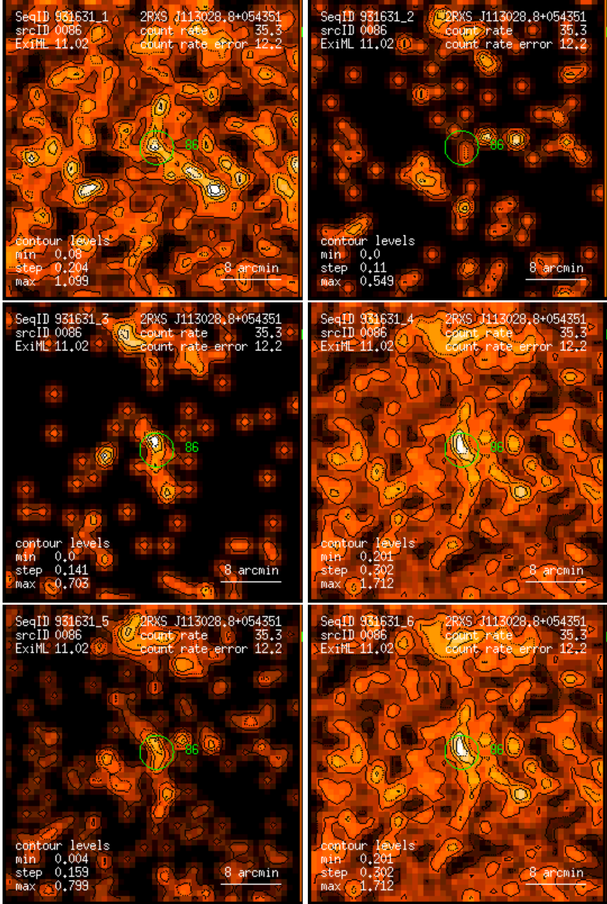
Figure 86: RASS 931631: detection 0086: band rate images, Gaussian filter: (1) PSPC channels 11 – 41, (2) 52 – 90, (3) 91 – 201, (4) 11 – 235, (5) 52 – 201, (6) 11 – 201. Broad band rates in counts/ks. Band rate contour levels in counts/ks/arcmin 2 .
