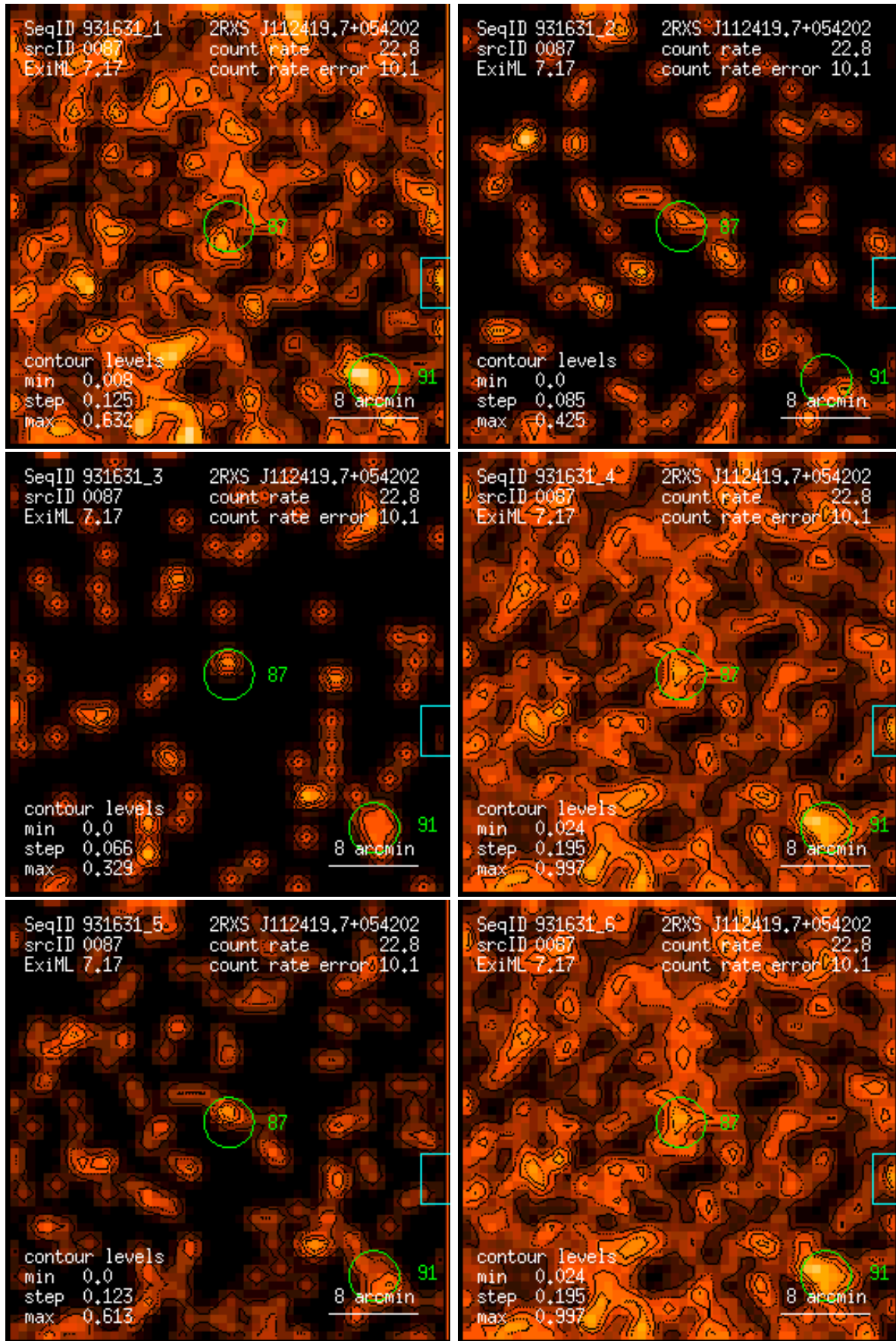
Figure 87: RASS 931631: detection 0087: band rate images, Gaussian filter: (1) PSPC channels 11 – 41, (2) 52 – 90, (3) 91 – 201, (4) 11 – 235, (5) 52 – 201, (6) 11 – 201. Broad band rates in counts/ks. Band rate contour levels in counts/ks/arcmin 2 .
