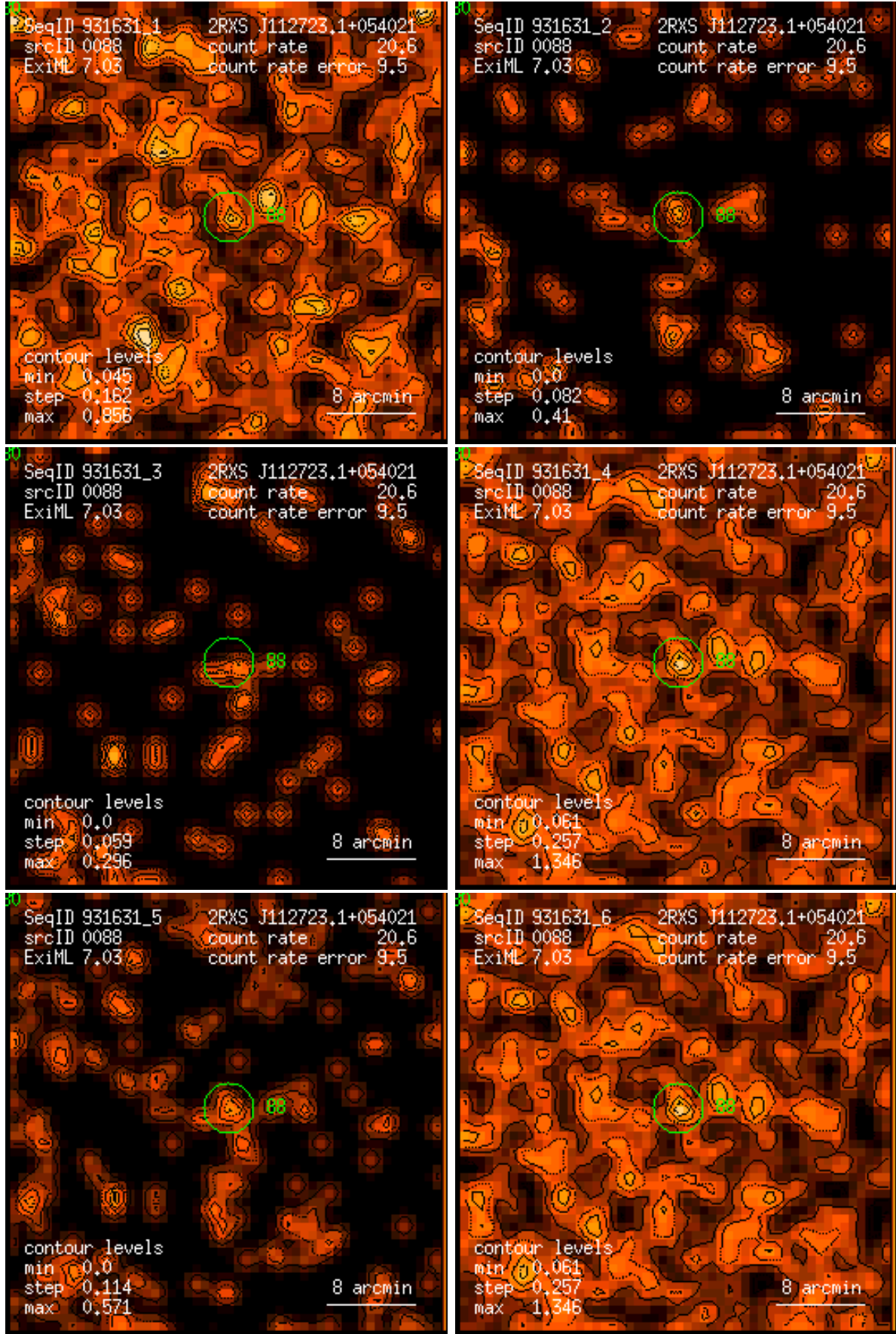
Figure 88: RASS 931631: detection 0088: band rate images, Gaussian filter: (1) PSPC channels 11 – 41, (2) 52 – 90, (3) 91 – 201, (4) 11 – 235, (5) 52 – 201, (6) 11 – 201. Broad band rates in counts/ks. Band rate contour levels in counts/ks/arcmin 2 .
