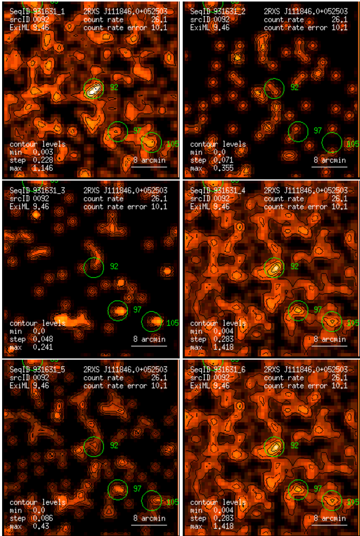
Figure 92: RASS 931631: detection 0092: band rate images, Gaussian filter: (1) PSPC channels 11 – 41, (2) 52 – 90, (3) 91 – 201, (4) 11 – 235, (5) 52 – 201, (6) 11 – 201. Broad band rates in counts/ks. Band rate contour levels in counts/ks/arcmin 2 .
