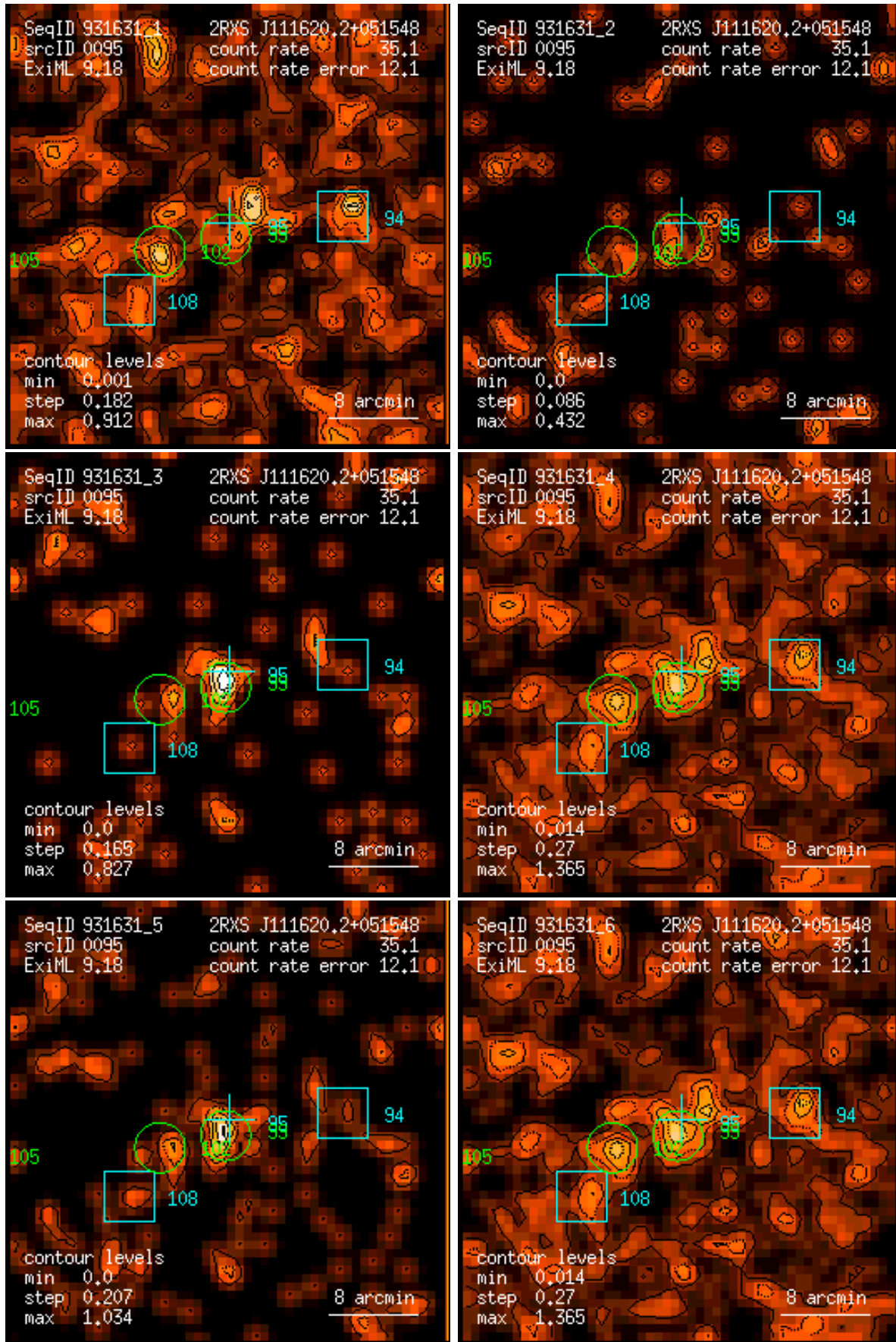
Figure 95: RASS 931631: detection 0095: band rate images, Gaussian filter: (1) PSPC channels 11 – 41, (2) 52 – 90, (3) 91 – 201, (4) 11 – 235, (5) 52 – 201, (6) 11 – 201. Broad band rates in counts/ks. Band rate contour levels in counts/ks/arcmin 2 .
