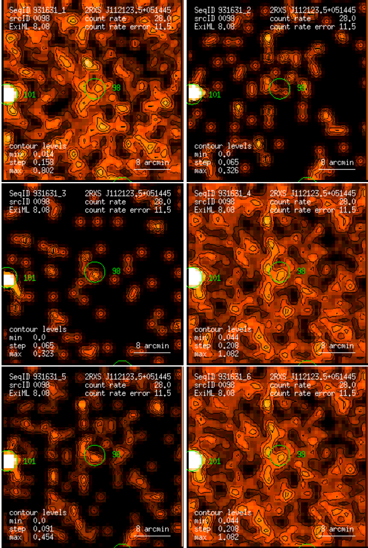
Figure 98: RASS 931631: detection 0098: band rate images, Gaussian filter: (1) PSPC channels 11 – 41, (2) 52 – 90, (3) 91 – 201, (4) 11 – 235, (5) 52 – 201, (6) 11 – 201. Broad band rates in counts/ks. Band rate contour levels in counts/ks/arcmin 2 .
