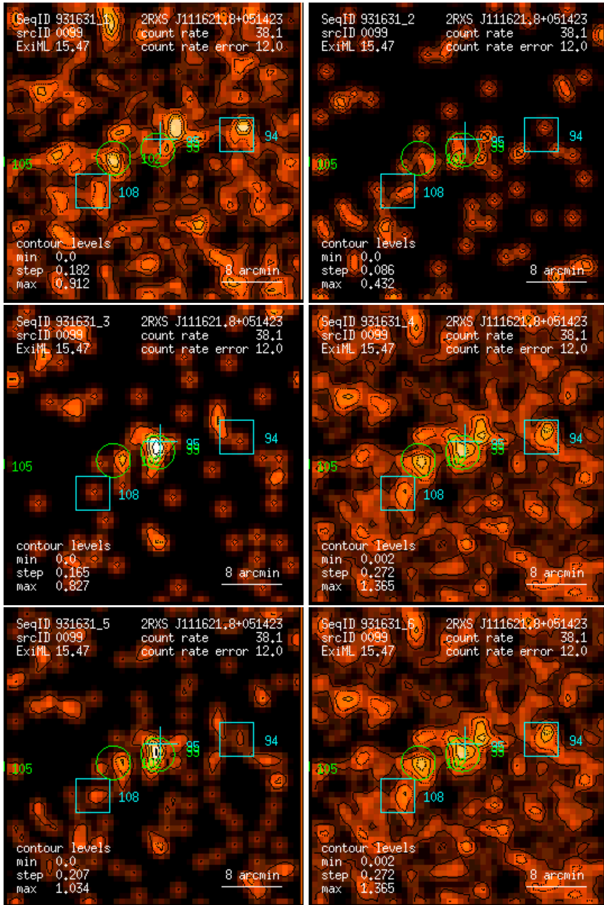
Figure 99: RASS 931631: detection 0099: band rate images, Gaussian filter: (1) PSPC channels 11 – 41, (2) 52 – 90, (3) 91 – 201, (4) 11 – 235, (5) 52 – 201, (6) 11 – 201. Broad band rates in counts/ks. Band rate contour levels in counts/ks/arcmin 2 .
