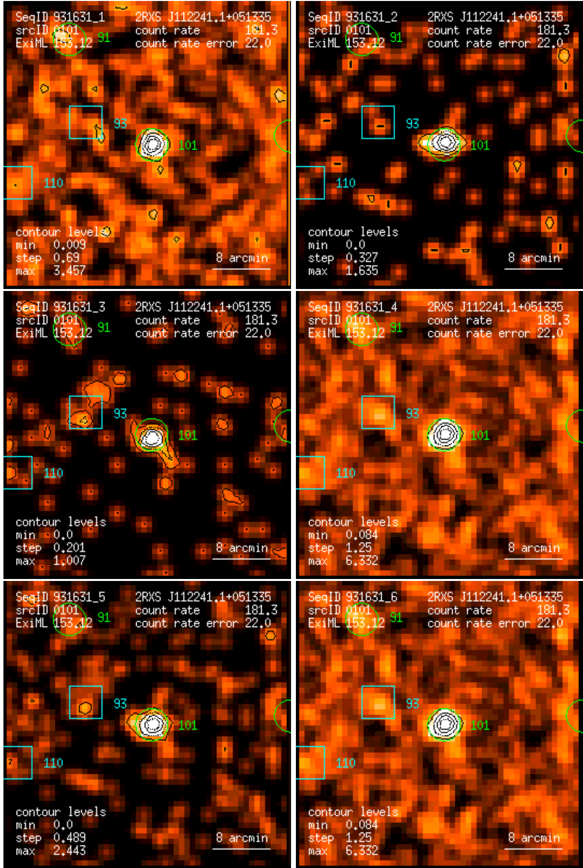
Figure 101: RASS 931631: detection 0101: band rate images, Gaussian filter: (1) PSPC channels 11 – 41, (2) 52 – 90, (3) 91 – 201, (4) 11 – 235, (5) 52 – 201, (6) 11 – 201. Broad band rates in counts/ks. Band rate contour levels in counts/ks/arcmin 2 .
