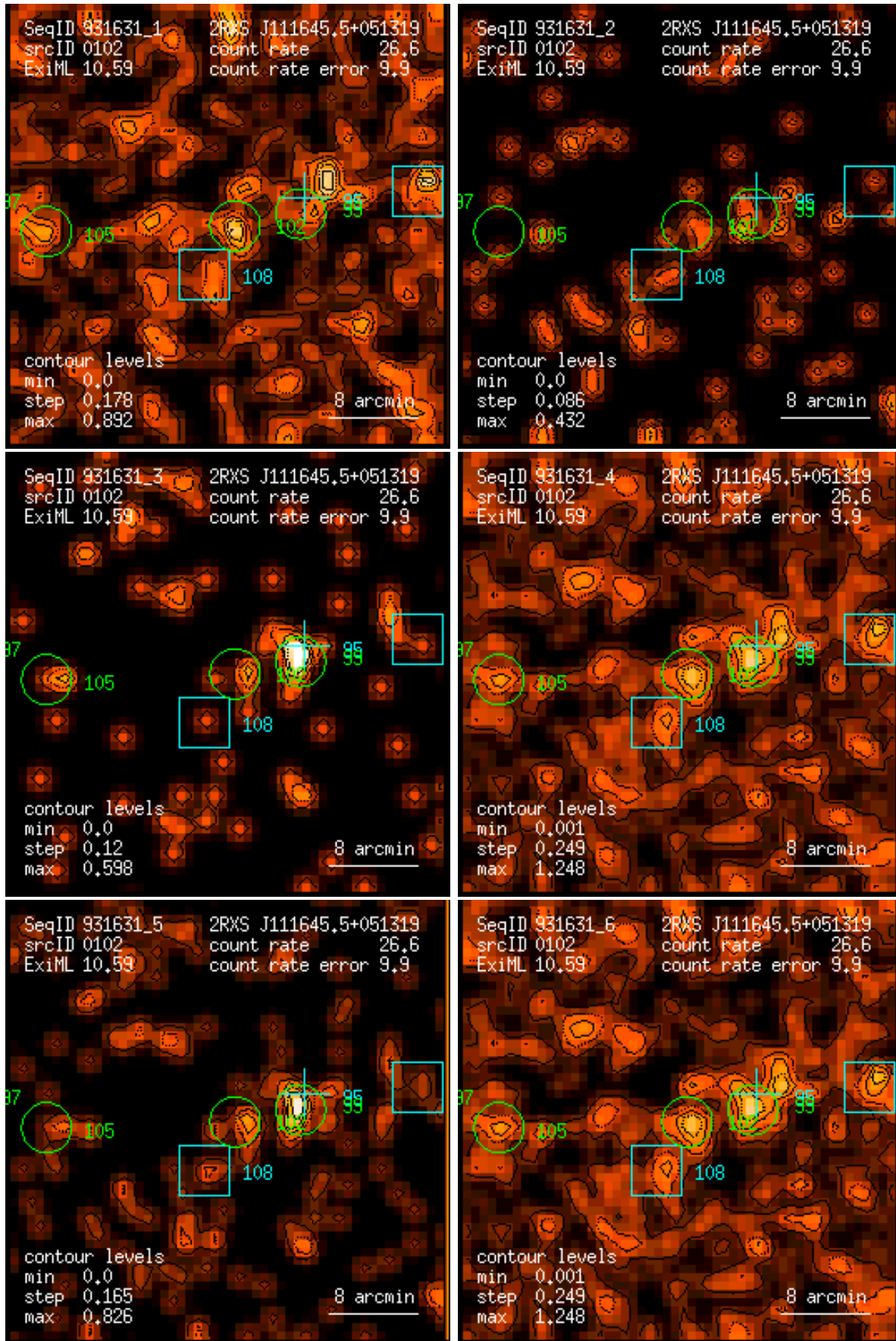
Figure 102: RASS 931631: detection 0102: band rate images, Gaussian filter: (1) PSPC channels 11 – 41, (2) 52 – 90, (3) 91 – 201, (4) 11 – 235, (5) 52 – 201, (6) 11 – 201. Broad band rates in counts/ks. Band rate contour levels in counts/ks/arcmin 2 .
