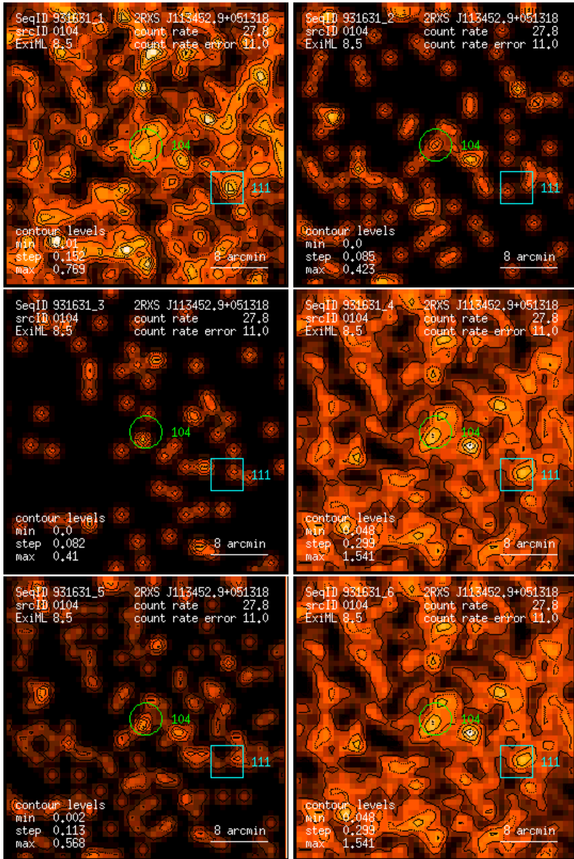
Figure 104: RASS 931631: detection 0104: band rate images, Gaussian filter: (1) PSPC channels 11 – 41, (2) 52 – 90, (3) 91 – 201, (4) 11 – 235, (5) 52 – 201, (6) 11 – 201. Broad band rates in counts/ks. Band rate contour levels in counts/ks/arcmin 2 .
