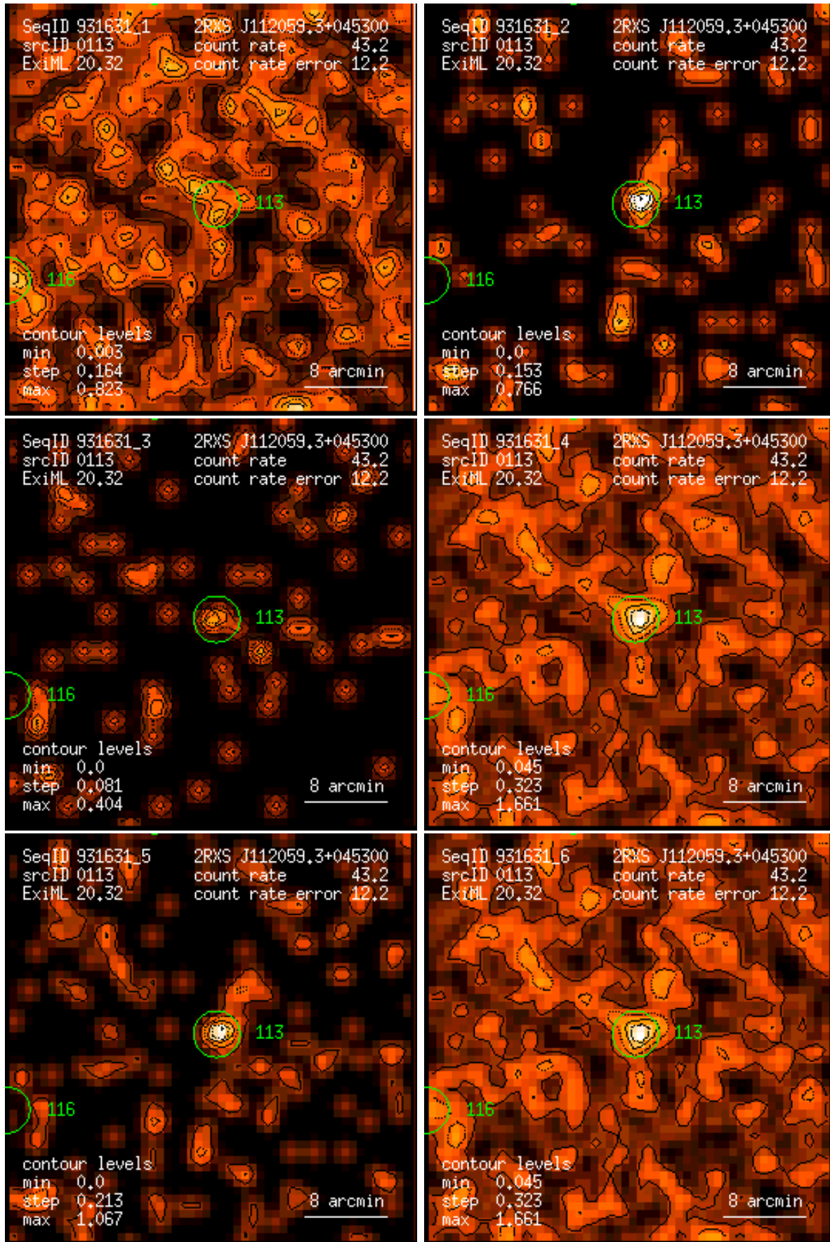
Figure 113: RASS 931631: detection 0113: band rate images, Gaussian filter: (1) PSPC channels 11 – 41, (2) 52 – 90, (3) 91 – 201, (4) 11 – 235, (5) 52 – 201, (6) 11 – 201. Broad band rates in counts/ks. Band rate contour levels in counts/ks/arcmin 2 .
