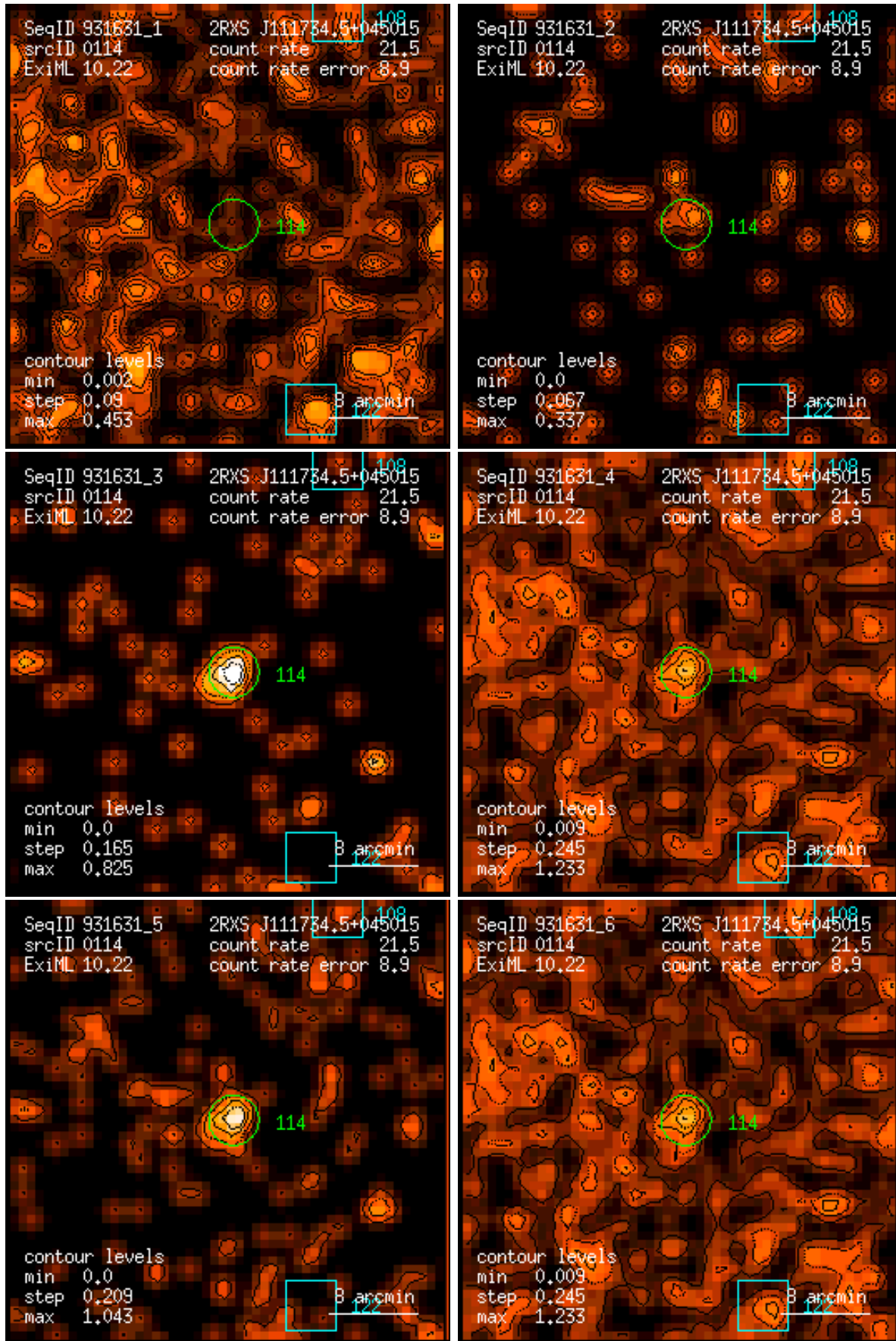
Figure 114: RASS 931631: detection 0114: band rate images, Gaussian filter: (1) PSPC channels 11 – 41, (2) 52 – 90, (3) 91 – 201, (4) 11 – 235, (5) 52 – 201, (6) 11 – 201. Broad band rates in counts/ks. Band rate contour levels in counts/ks/arcmin 2 .
