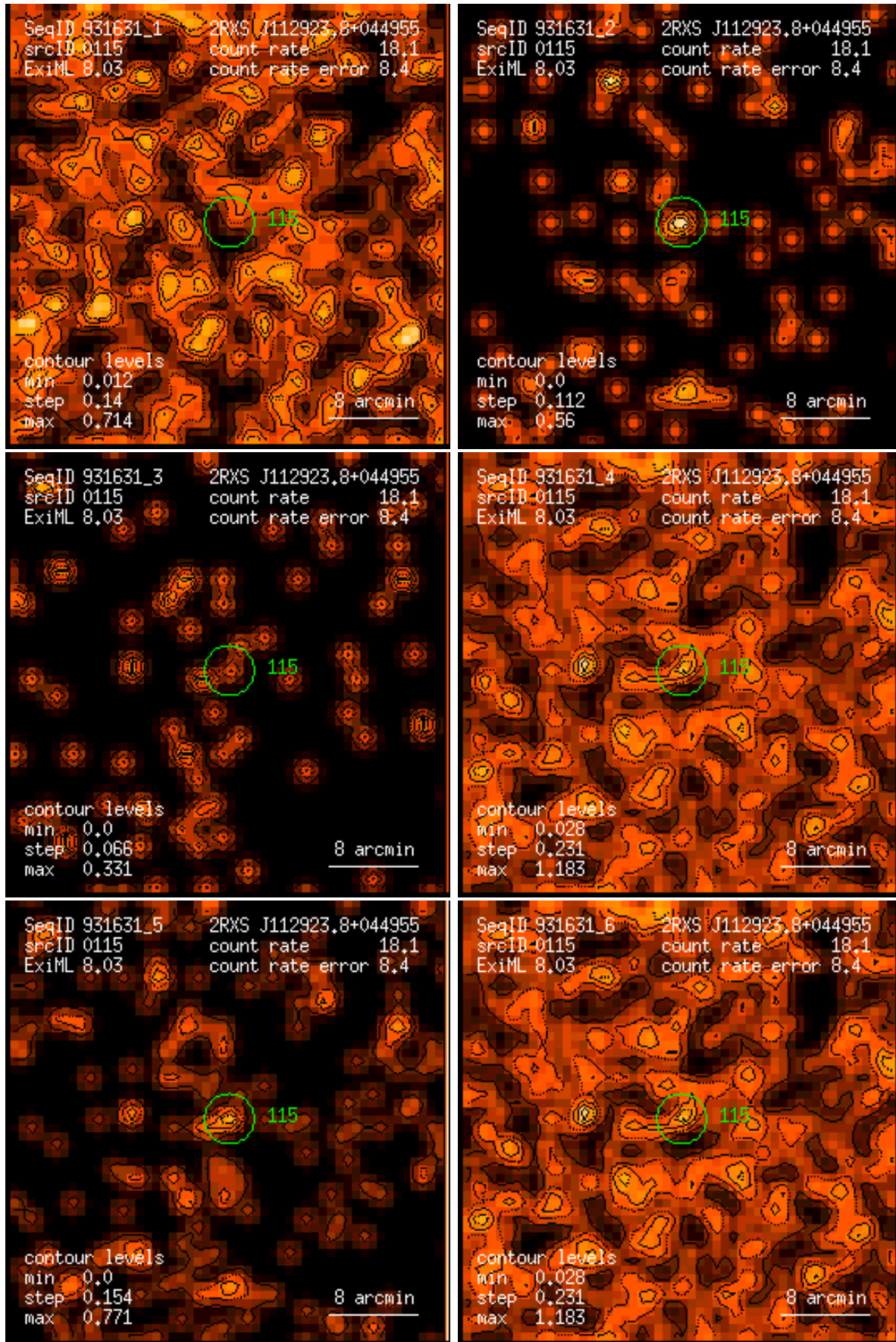
Figure 115: RASS 931631: detection 0115: band rate images, Gaussian filter: (1) PSPC channels 11 – 41, (2) 52 – 90, (3) 91 – 201, (4) 11 – 235, (5) 52 – 201, (6) 11 – 201. Broad band rates in counts/ks. Band rate contour levels in counts/ks/arcmin 2 .
