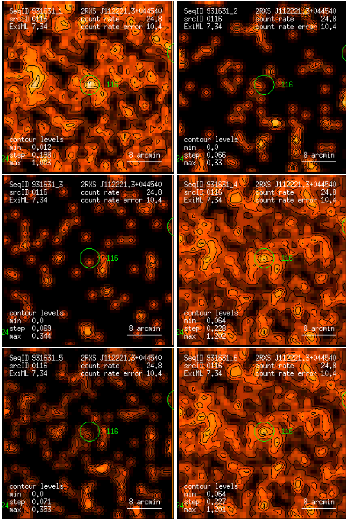
Figure 116: RASS 931631: detection 0116: band rate images, Gaussian filter: (1) PSPC channels 11 – 41, (2) 52 – 90, (3) 91 – 201, (4) 11 – 235, (5) 52 – 201, (6) 11 – 201. Broad band rates in counts/ks. Band rate contour levels in counts/ks/arcmin 2 .
