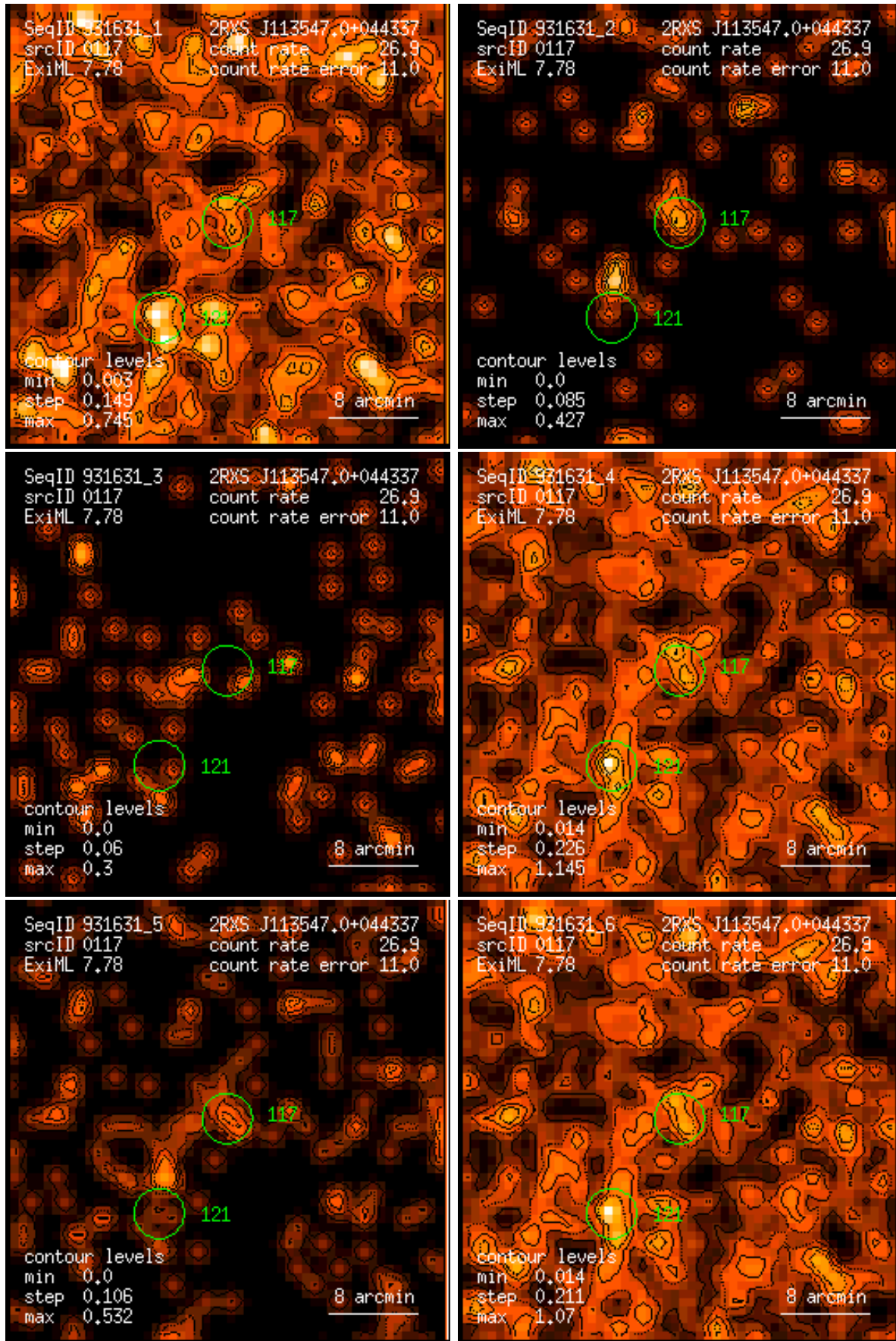
Figure 117: RASS 931631: detection 0117: band rate images, Gaussian filter: (1) PSPC channels 11 – 41, (2) 52 – 90, (3) 91 – 201, (4) 11 – 235, (5) 52 – 201, (6) 11 – 201. Broad band rates in counts/ks. Band rate contour levels in counts/ks/arcmin 2 .
