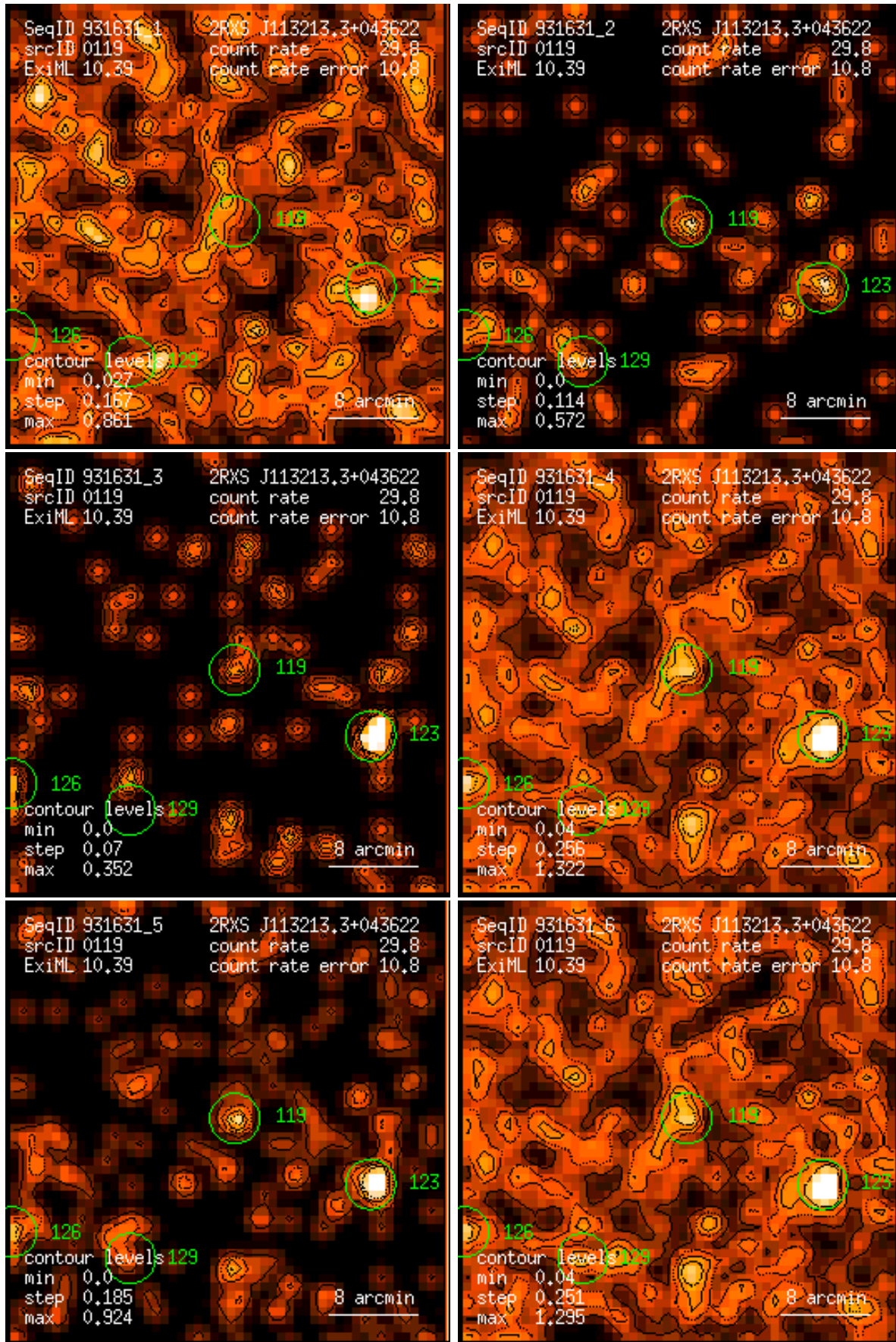
Figure 119: RASS 931631: detection 0119: band rate images, Gaussian filter: (1) PSPC channels 11 – 41, (2) 52 – 90, (3) 91 – 201, (4) 11 – 235, (5) 52 – 201, (6) 11 – 201. Broad band rates in counts/ks. Band rate contour levels in counts/ks/arcmin 2 .
