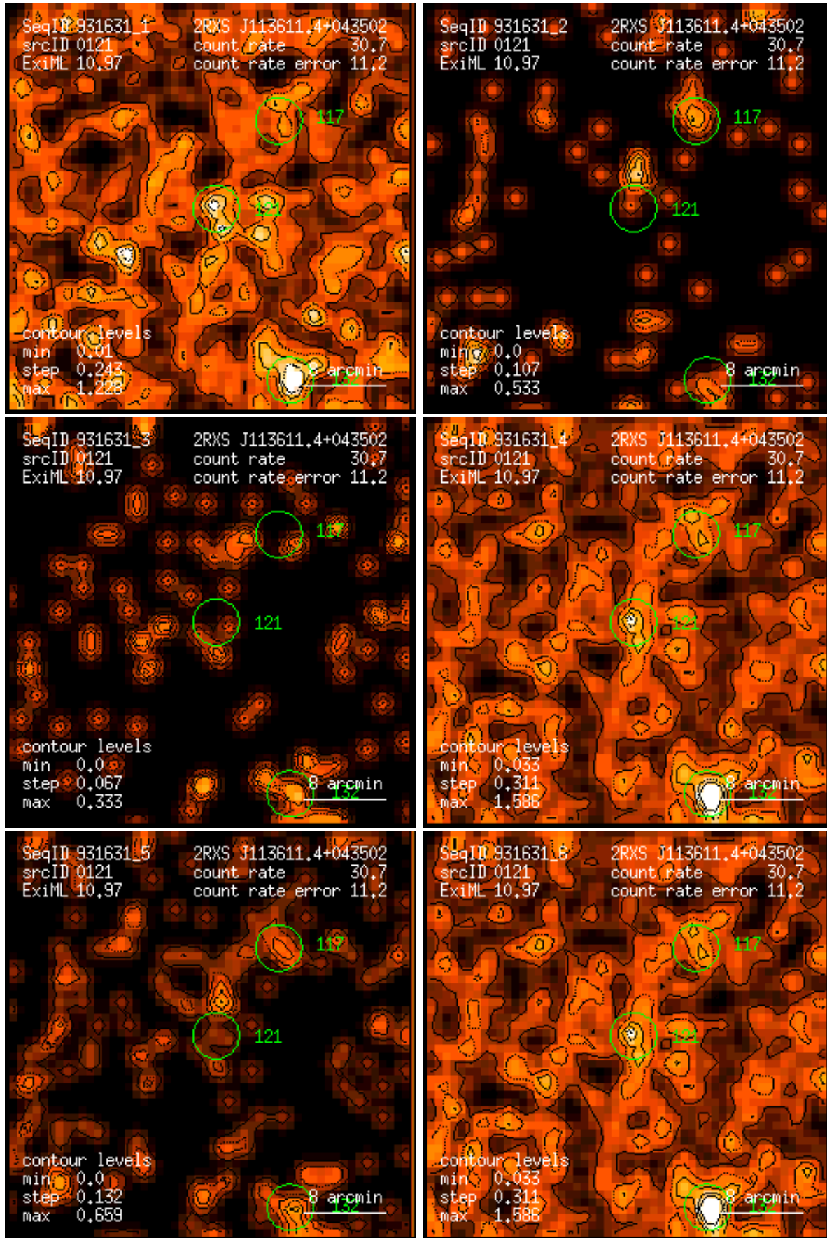
Figure 121: RASS 931631: detection 0121: band rate images, Gaussian filter: (1) PSPC channels 11 – 41, (2) 52 – 90, (3) 91 – 201, (4) 11 – 235, (5) 52 – 201, (6) 11 – 201. Broad band rates in counts/ks. Band rate contour levels in counts/ks/arcmin 2 .
