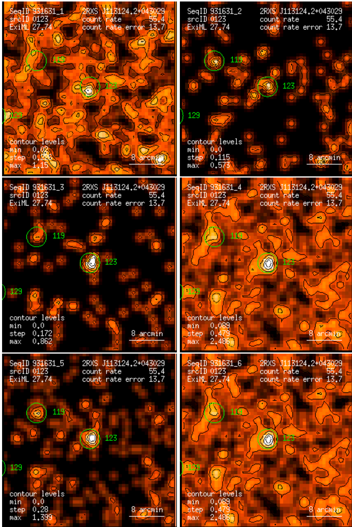
Figure 123: RASS 931631: detection 0123: band rate images, Gaussian filter: (1) PSPC channels 11 – 41, (2) 52 – 90, (3) 91 – 201, (4) 11 – 235, (5) 52 – 201, (6) 11 – 201. Broad band rates in counts/ks. Band rate contour levels in counts/ks/arcmin 2 .
