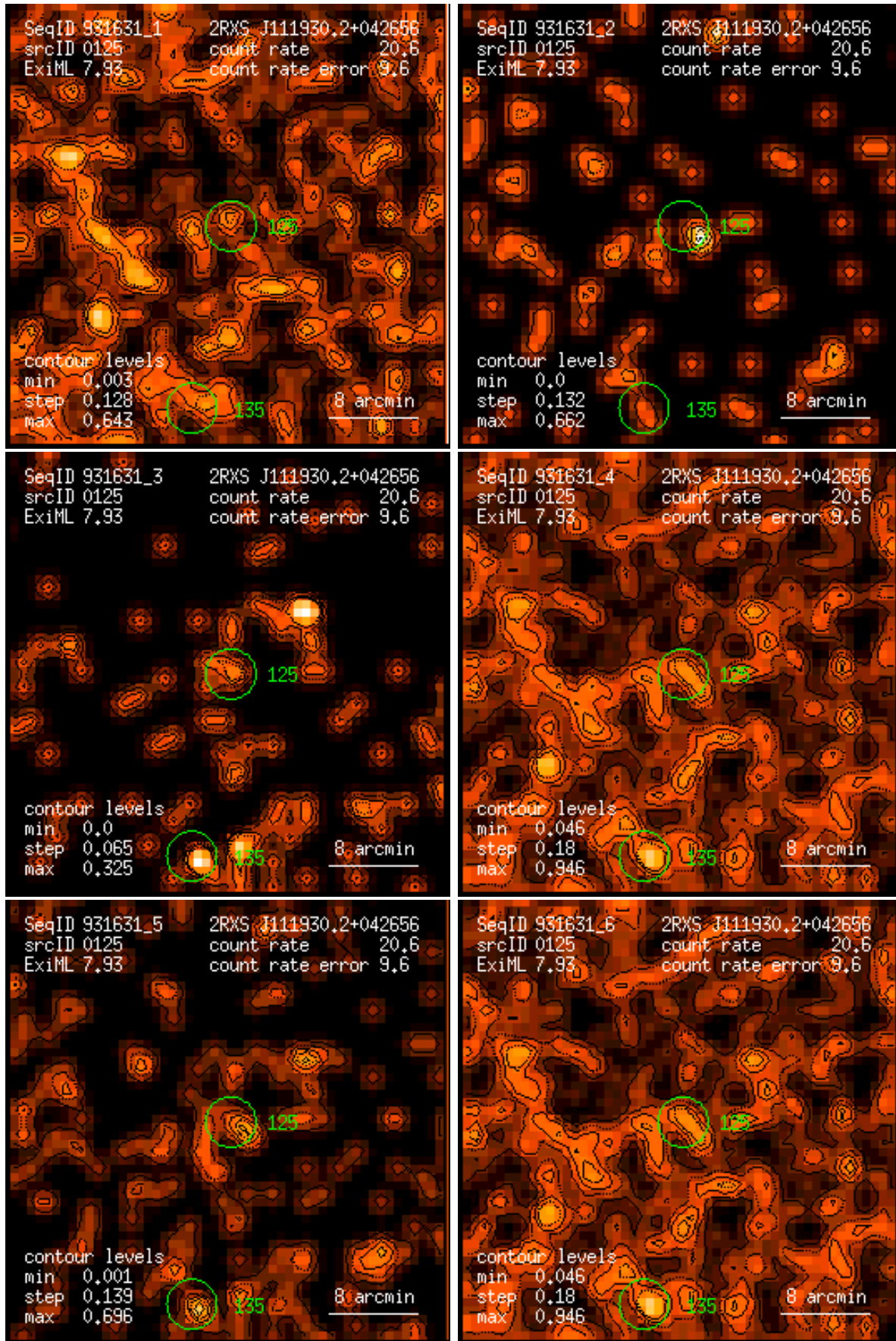
Figure 125: RASS 931631: detection 0125: band rate images, Gaussian filter: (1) PSPC channels 11 – 41, (2) 52 – 90, (3) 91 – 201, (4) 11 – 235, (5) 52 – 201, (6) 11 – 201. Broad band rates in counts/ks. Band rate contour levels in counts/ks/arcmin 2 .
