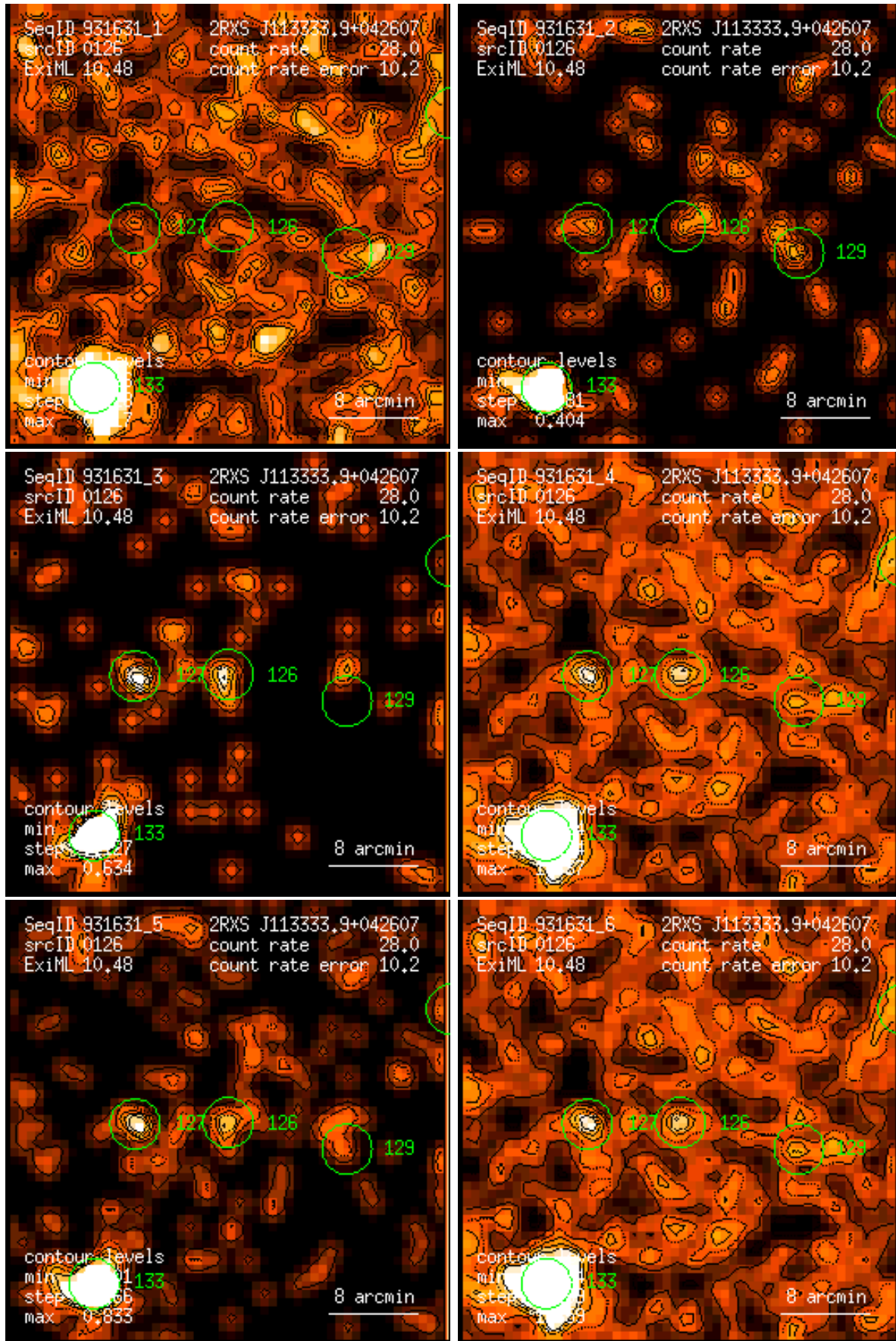
Figure 126: RASS 931631: detection 0126: band rate images, Gaussian filter: (1) PSPC channels 11 – 41, (2) 52 – 90, (3) 91 – 201, (4) 11 – 235, (5) 52 – 201, (6) 11 – 201. Broad band rates in counts/ks. Band rate contour levels in counts/ks/arcmin 2 .
