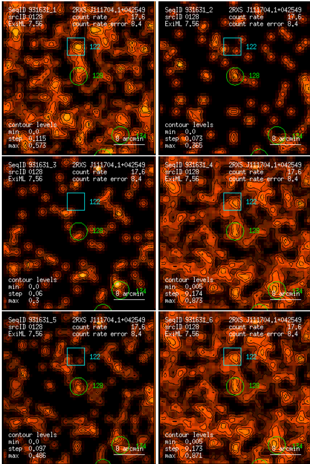
Figure 128: RASS 931631: detection 0128: band rate images, Gaussian filter: (1) PSPC channels 11 – 41, (2) 52 – 90, (3) 91 – 201, (4) 11 – 235, (5) 52 – 201, (6) 11 – 201. Broad band rates in counts/ks. Band rate contour levels in counts/ks/arcmin 2 .
