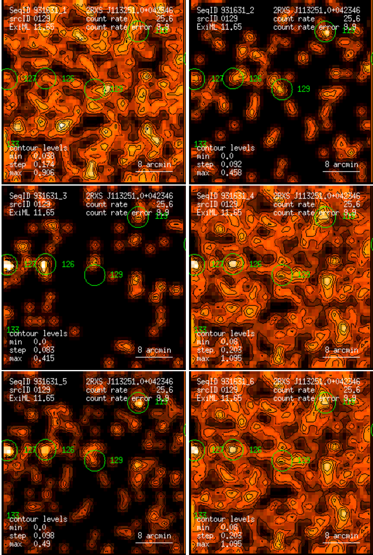
Figure 129: RASS 931631: detection 0129: band rate images, Gaussian filter: (1) PSPC channels 11 – 41, (2) 52 – 90, (3) 91 – 201, (4) 11 – 235, (5) 52 – 201, (6) 11 – 201. Broad band rates in counts/ks. Band rate contour levels in counts/ks/arcmin 2 .
