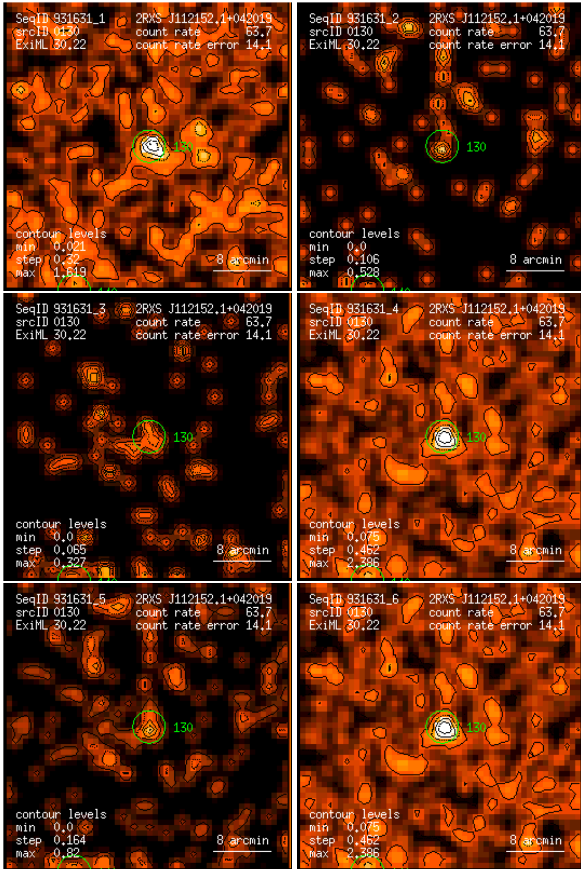
Figure 130: RASS 931631: detection 0130: band rate images, Gaussian filter: (1) PSPC channels 11 – 41, (2) 52 – 90, (3) 91 – 201, (4) 11 – 235, (5) 52 – 201, (6) 11 – 201. Broad band rates in counts/ks. Band rate contour levels in counts/ks/arcmin 2 .
