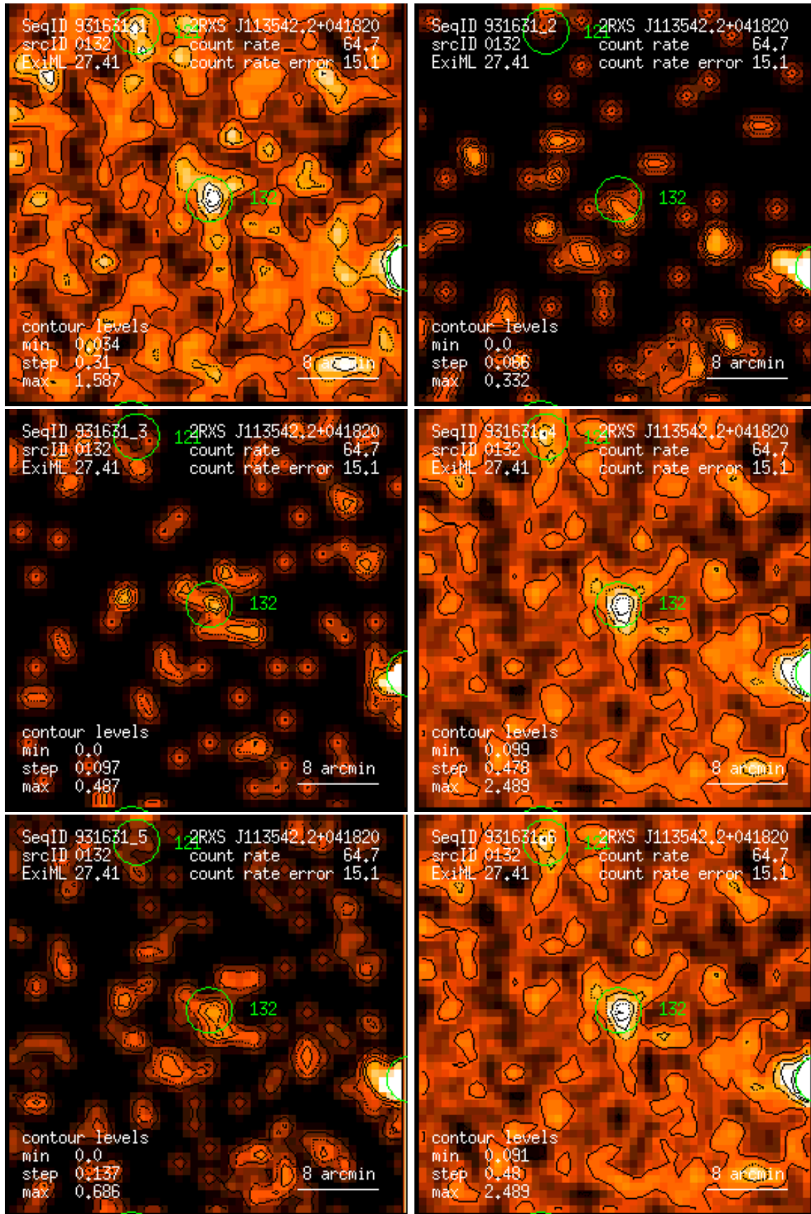
Figure 132: RASS 931631: detection 0132: band rate images, Gaussian filter: (1) PSPC channels 11 – 41, (2) 52 – 90, (3) 91 – 201, (4) 11 – 235, (5) 52 – 201, (6) 11 – 201. Broad band rates in counts/ks. Band rate contour levels in counts/ks/arcmin 2 .
