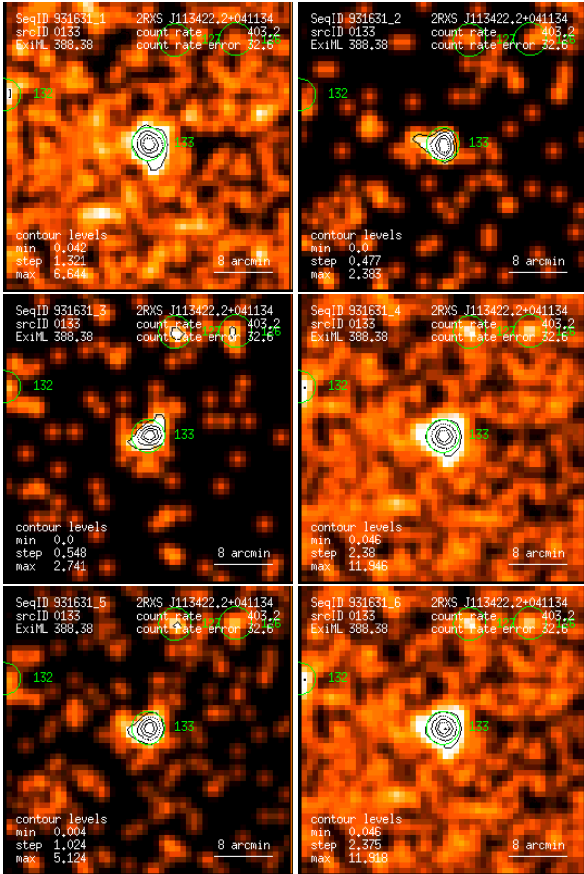
Figure 133: RASS 931631: detection 0133: band rate images, Gaussian filter: (1) PSPC channels 11 – 41, (2) 52 – 90, (3) 91 – 201, (4) 11 – 235, (5) 52 – 201, (6) 11 – 201. Broad band rates in counts/ks. Band rate contour levels in counts/ks/arcmin 2 .
