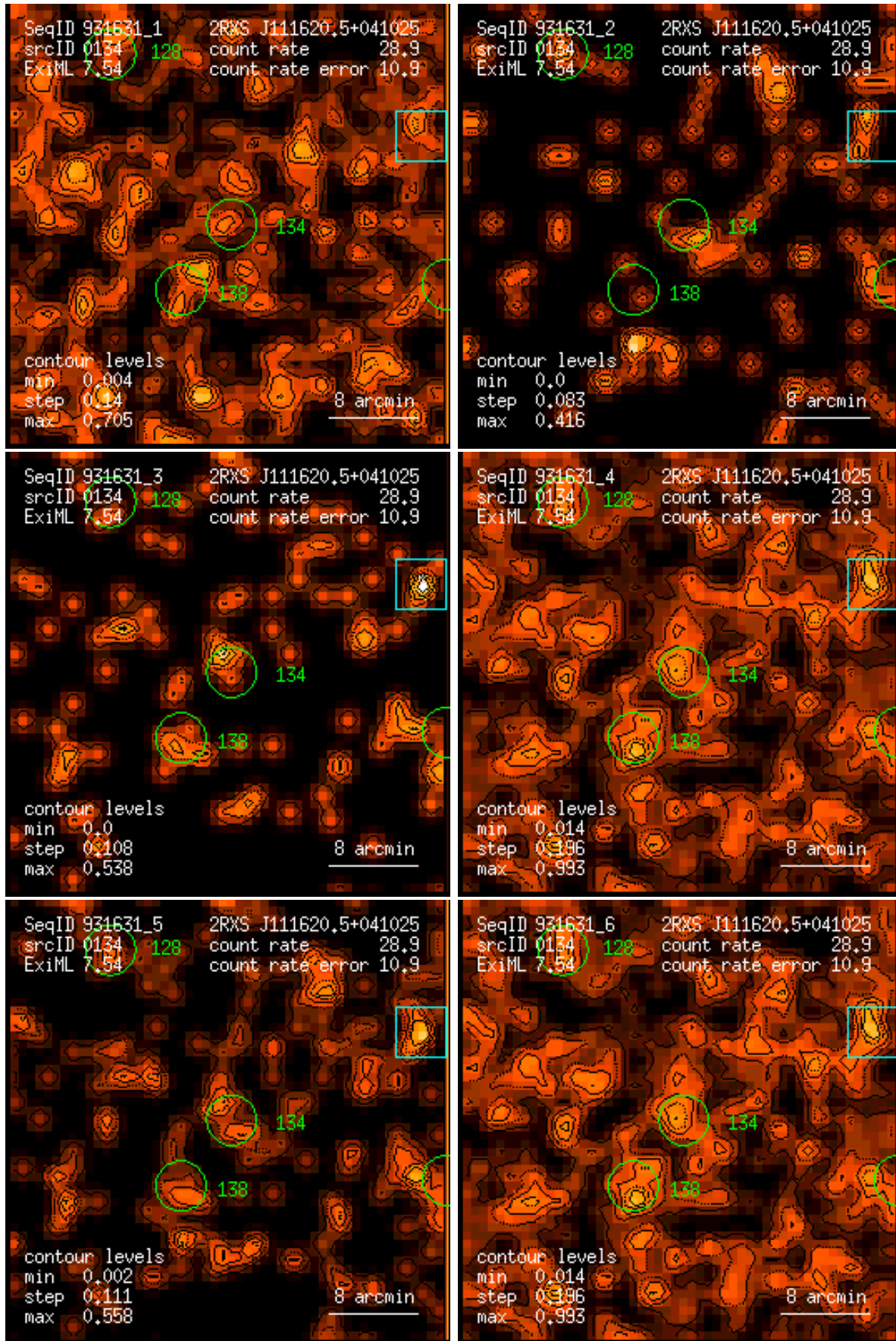
Figure 134: RASS 931631: detection 0134: band rate images, Gaussian filter: (1) PSPC channels 11 – 41, (2) 52 – 90, (3) 91 – 201, (4) 11 – 235, (5) 52 – 201, (6) 11 – 201. Broad band rates in counts/ks. Band rate contour levels in counts/ks/arcmin 2 .
