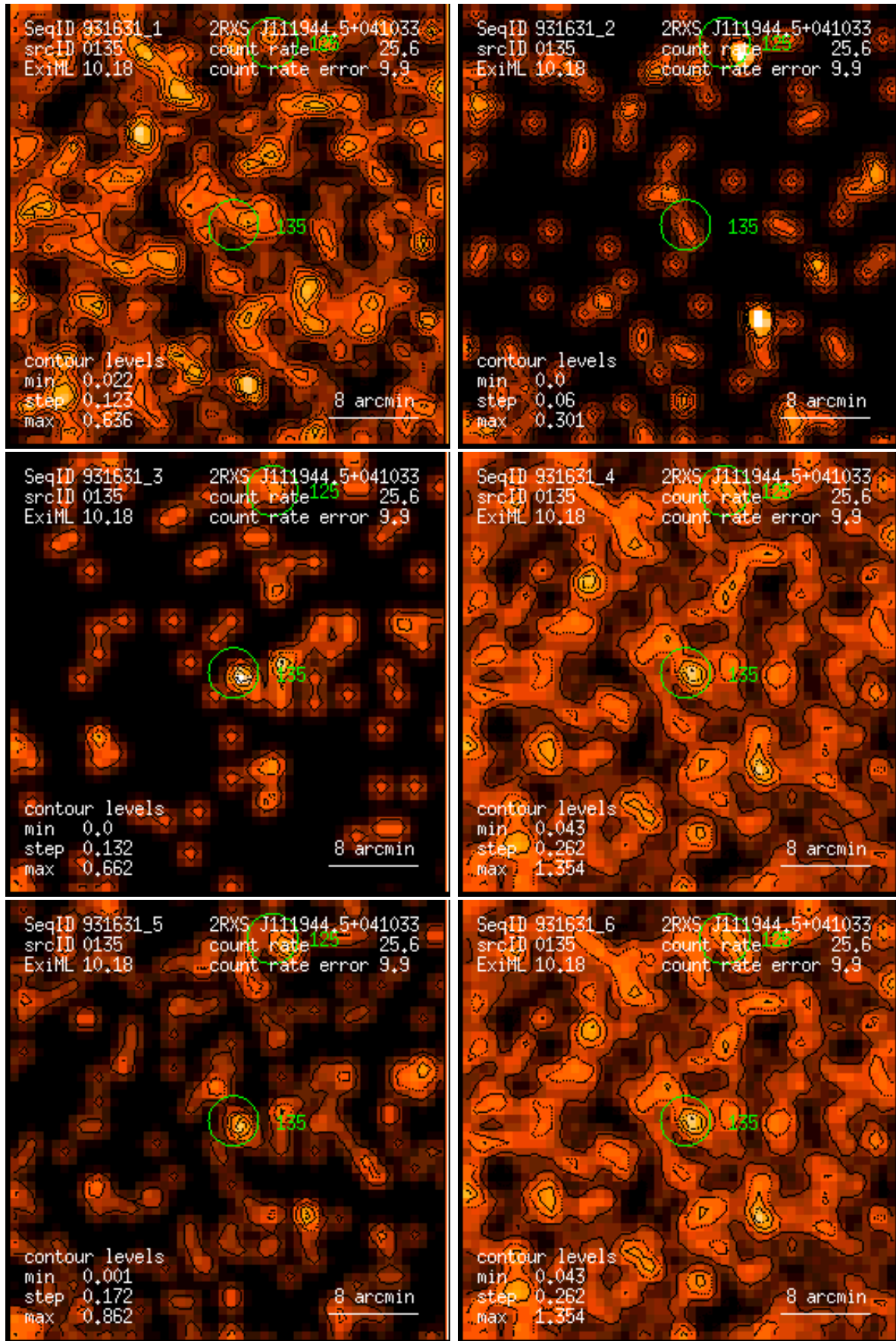
Figure 135: RASS 931631: detection 0135: band rate images, Gaussian filter: (1) PSPC channels 11 – 41, (2) 52 – 90, (3) 91 – 201, (4) 11 – 235, (5) 52 – 201, (6) 11 – 201. Broad band rates in counts/ks. Band rate contour levels in counts/ks/arcmin 2 .
