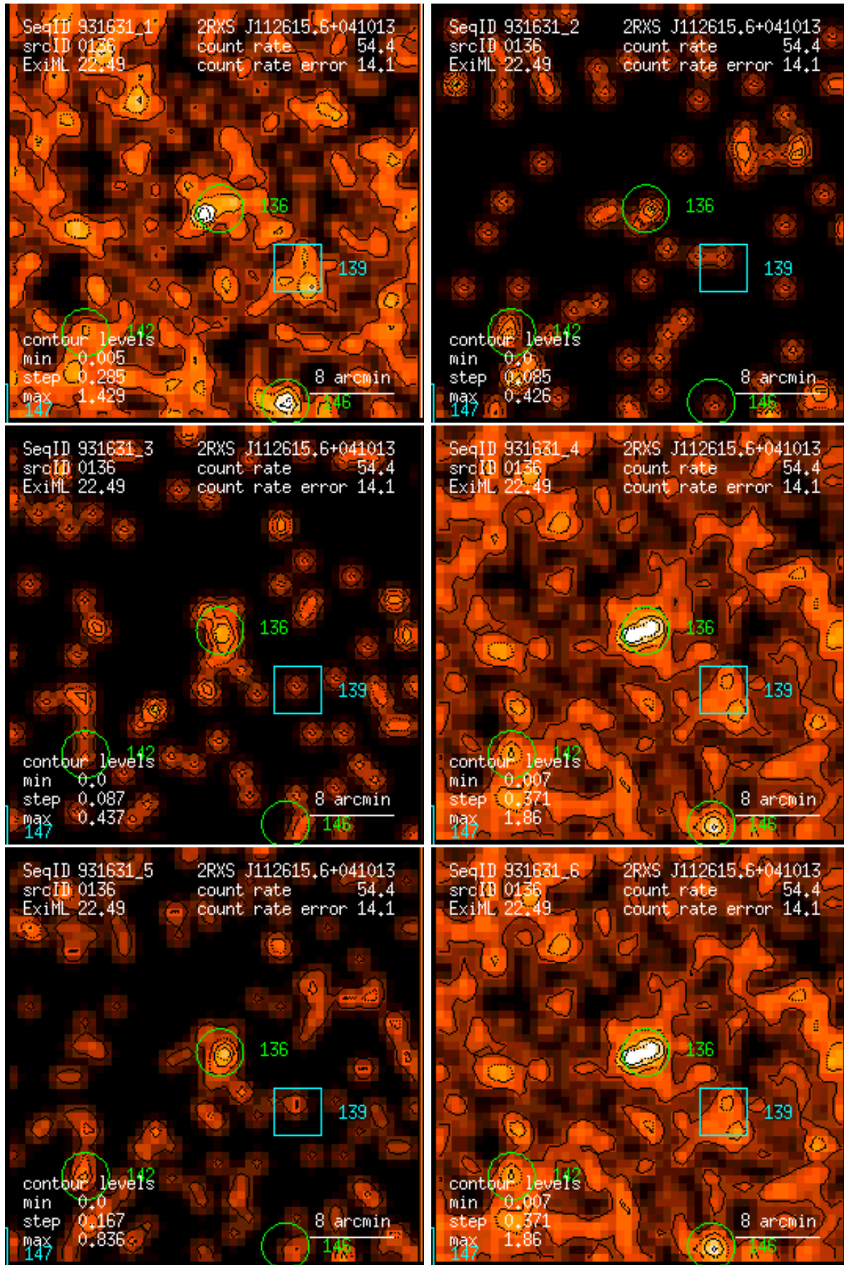
Figure 136: RASS 931631: detection 0136: band rate images, Gaussian filter: (1) PSPC channels 11 – 41, (2) 52 – 90, (3) 91 – 201, (4) 11 – 235, (5) 52 – 201, (6) 11 – 201. Broad band rates in counts/ks. Band rate contour levels in counts/ks/arcmin 2 .
