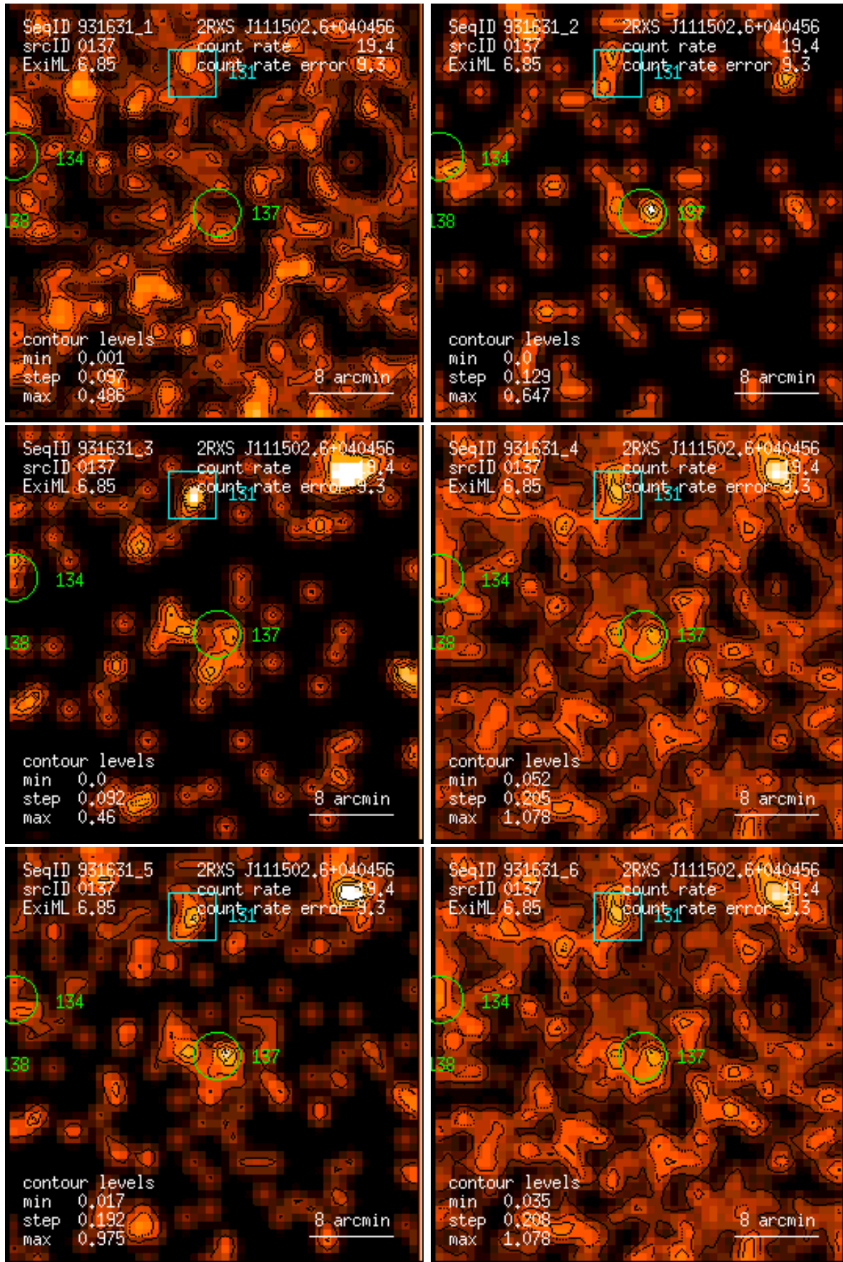
Figure 137: RASS 931631: detection 0137: band rate images, Gaussian filter: (1) PSPC channels 11 – 41, (2) 52 – 90, (3) 91 – 201, (4) 11 – 235, (5) 52 – 201, (6) 11 – 201. Broad band rates in counts/ks. Band rate contour levels in counts/ks/arcmin 2 .
