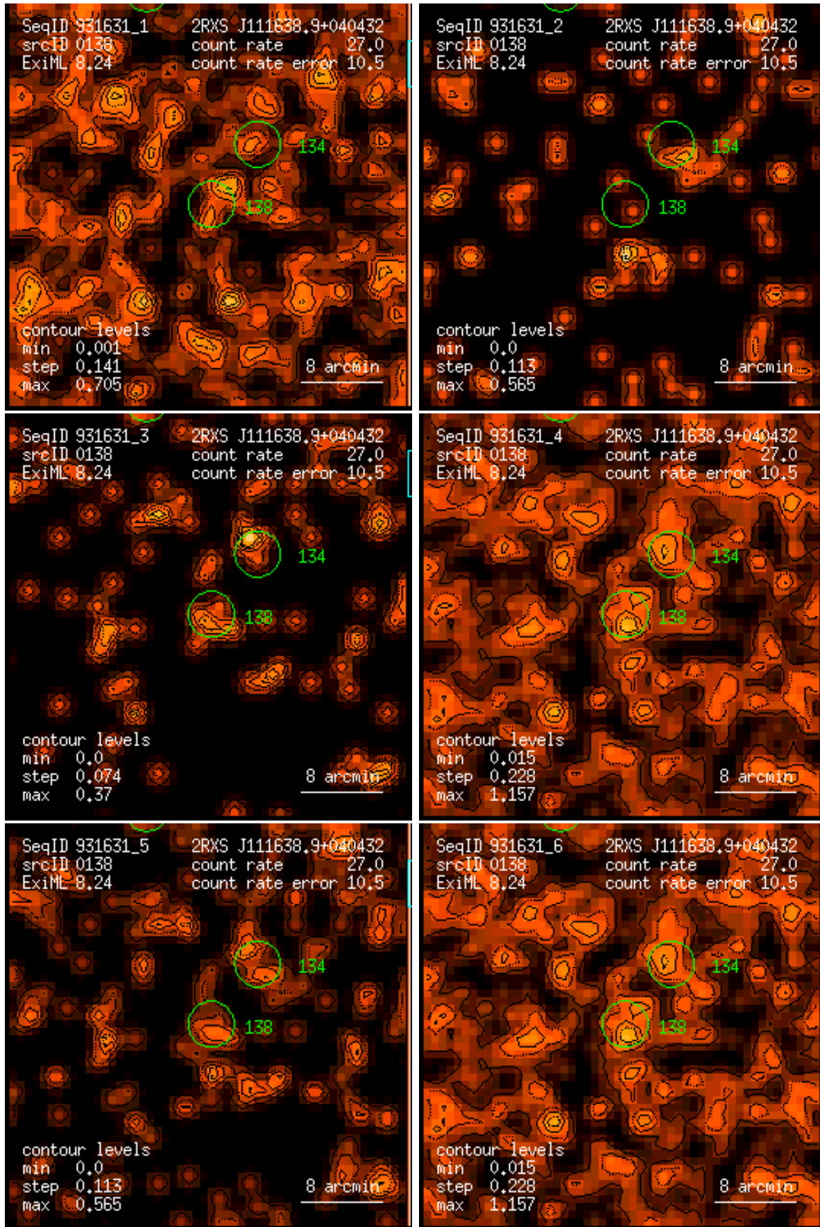
Figure 138: RASS 931631: detection 0138: band rate images, Gaussian filter: (1) PSPC channels 11 – 41, (2) 52 – 90, (3) 91 – 201, (4) 11 – 235, (5) 52 – 201, (6) 11 – 201. Broad band rates in counts/ks. Band rate contour levels in counts/ks/arcmin 2 .
