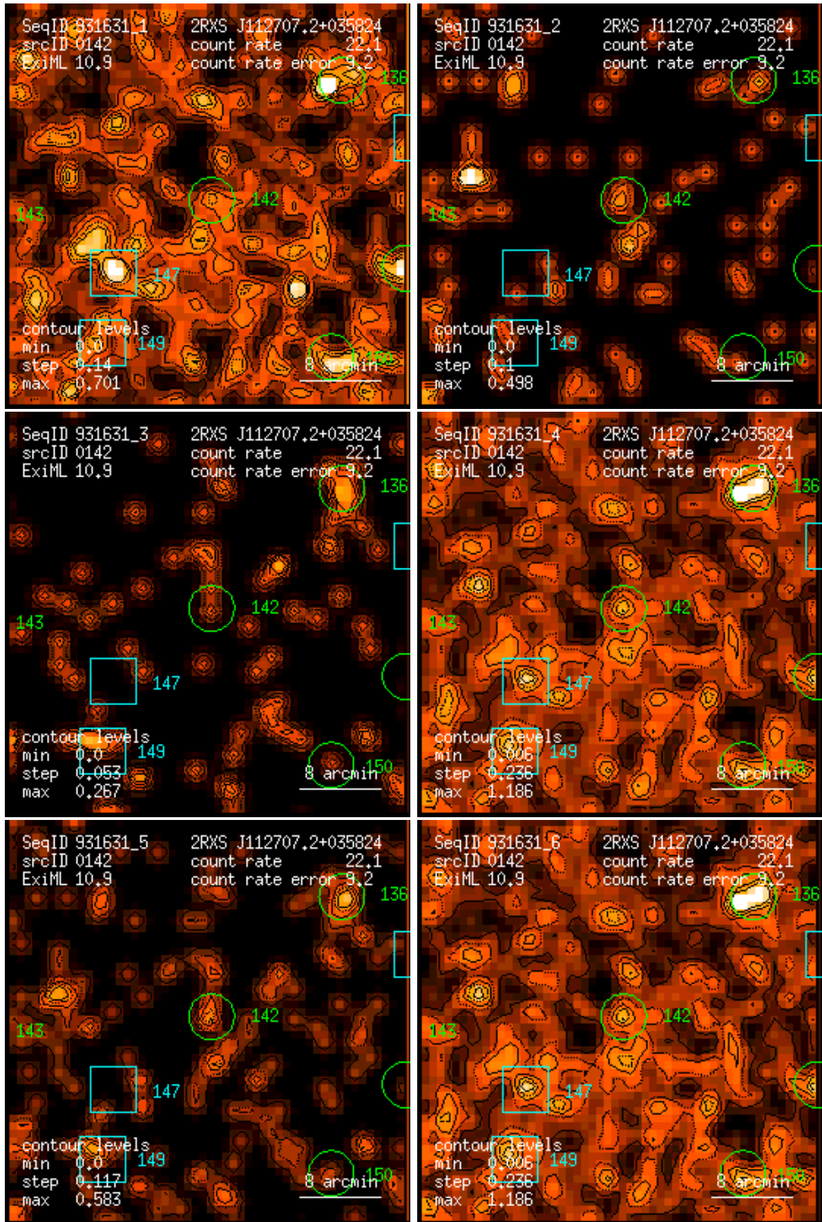
Figure 142: RASS 931631: detection 0142: band rate images, Gaussian filter: (1) PSPC channels 11 – 41, (2) 52 – 90, (3) 91 – 201, (4) 11 – 235, (5) 52 – 201, (6) 11 – 201. Broad band rates in counts/ks. Band rate contour levels in counts/ks/arcmin 2 .
