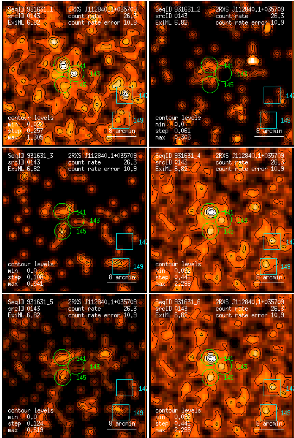
Figure 143: RASS 931631: detection 0143: band rate images, Gaussian filter: (1) PSPC channels 11 – 41, (2) 52 – 90, (3) 91 – 201, (4) 11 – 235, (5) 52 – 201, (6) 11 – 201. Broad band rates in counts/ks. Band rate contour levels in counts/ks/arcmin 2 .
