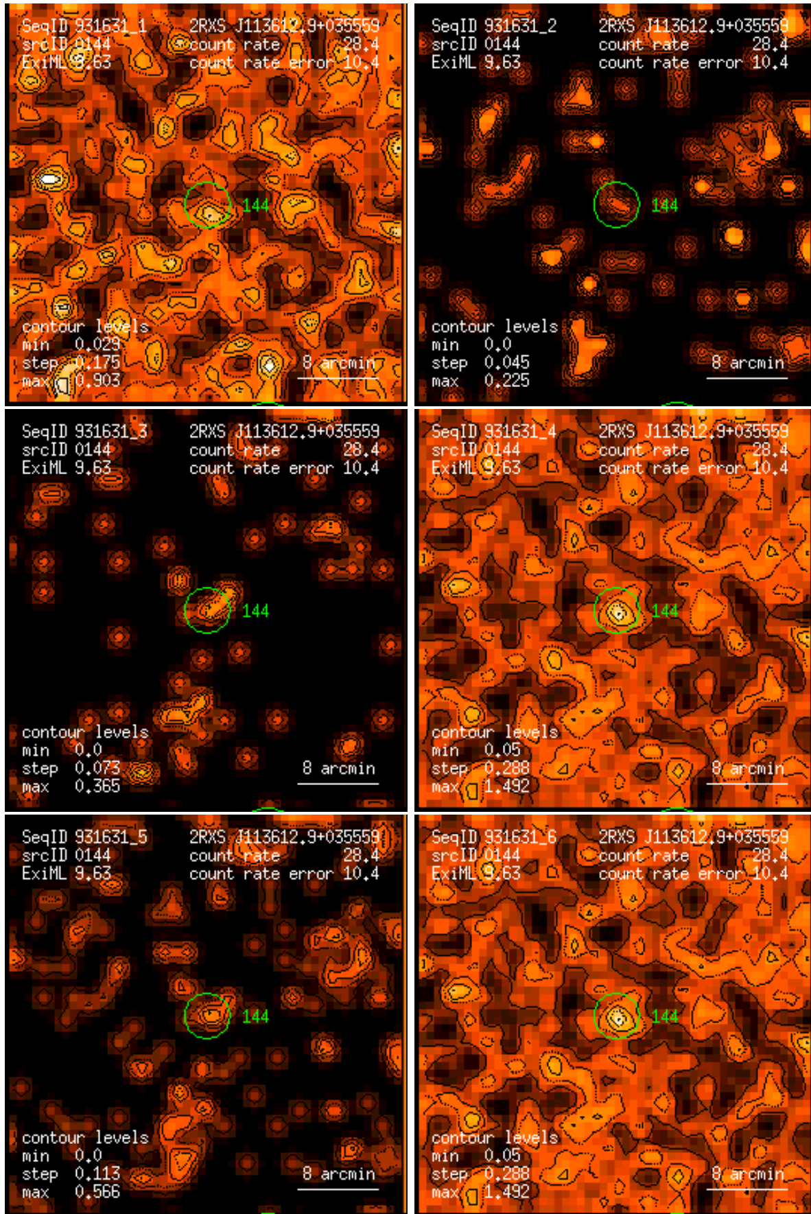
Figure 144: RASS 931631: detection 0144: band rate images, Gaussian filter: (1) PSPC channels 11 – 41, (2) 52 – 90, (3) 91 – 201, (4) 11 – 235, (5) 52 – 201, (6) 11 – 201. Broad band rates in counts/ks. Band rate contour levels in counts/ks/arcmin 2 .
