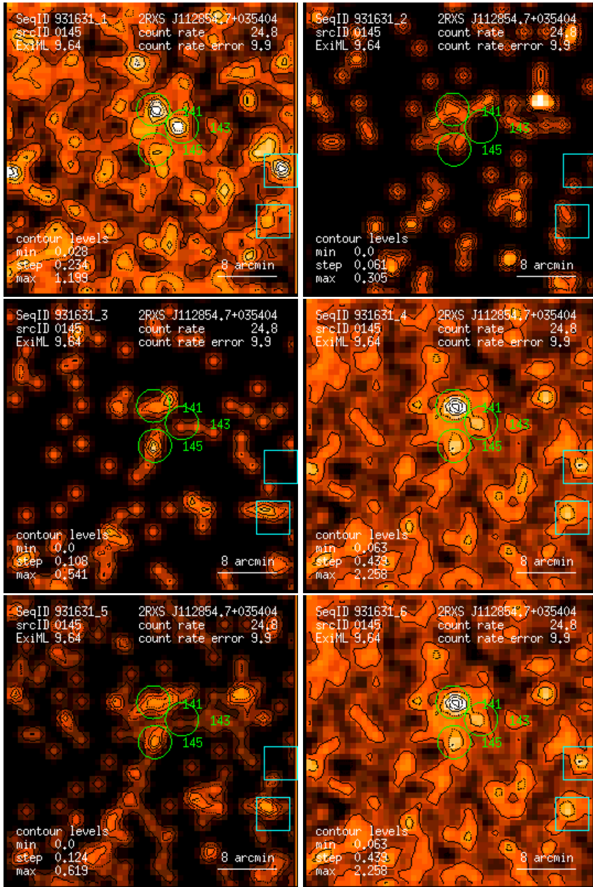
Figure 145: RASS 931631: detection 0145: band rate images, Gaussian filter: (1) PSPC channels 11 – 41, (2) 52 – 90, (3) 91 – 201, (4) 11 – 235, (5) 52 – 201, (6) 11 – 201. Broad band rates in counts/ks. Band rate contour levels in counts/ks/arcmin 2 .
