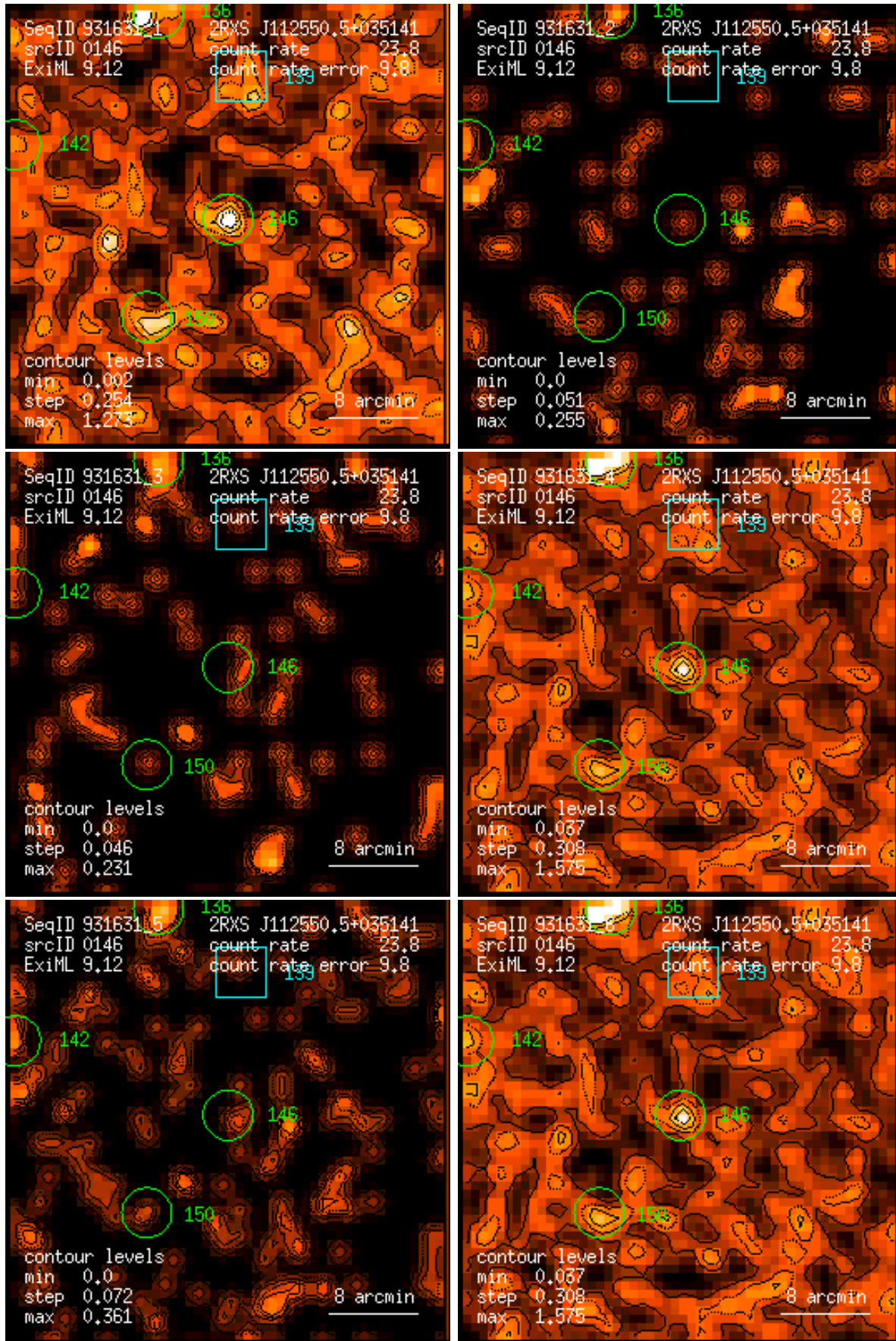
Figure 146: RASS 931631: detection 0146: band rate images, Gaussian filter: (1) PSPC channels 11 – 41, (2) 52 – 90, (3) 91 – 201, (4) 11 – 235, (5) 52 – 201, (6) 11 – 201. Broad band rates in counts/ks. Band rate contour levels in counts/ks/arcmin 2 .
