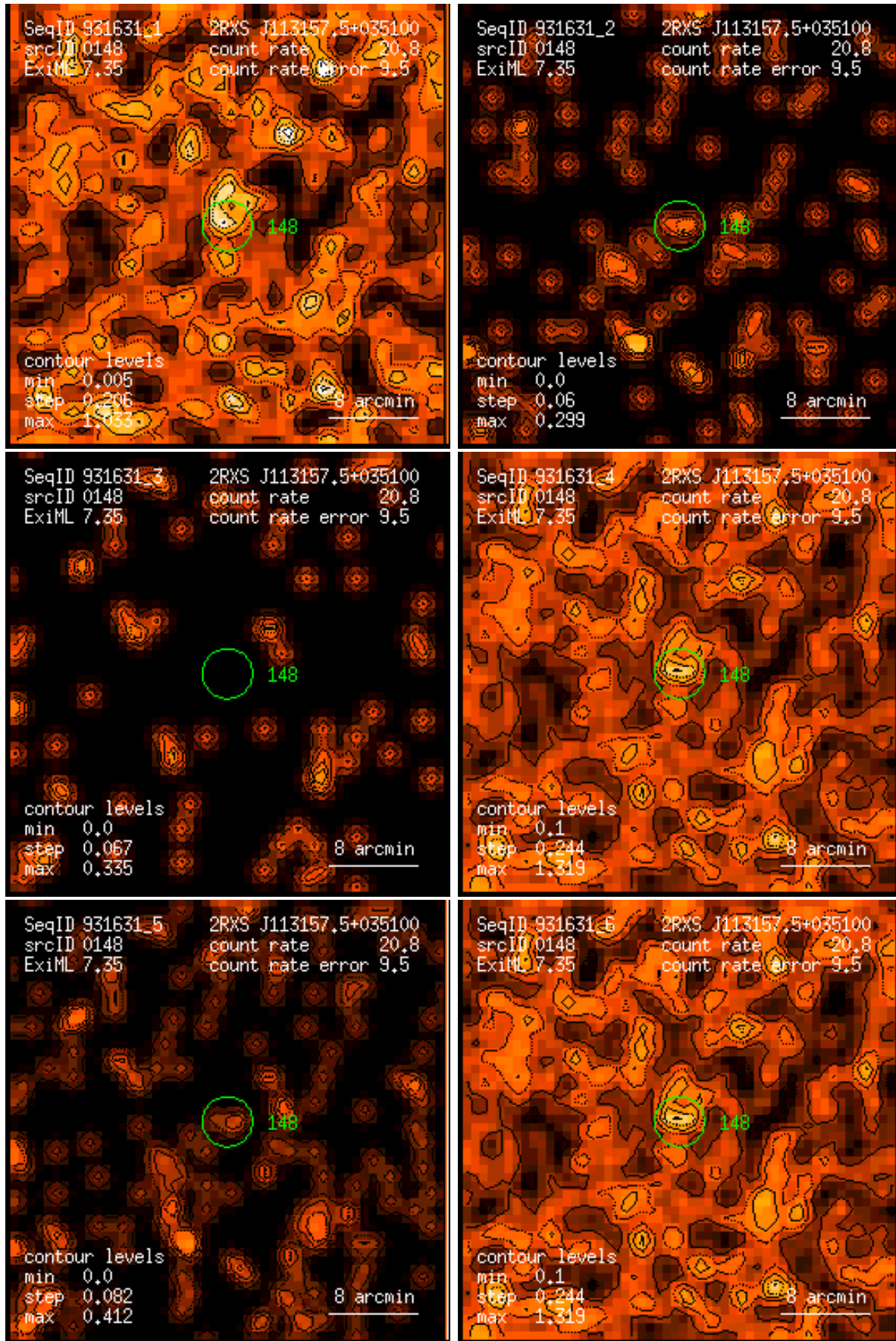
Figure 148: RASS 931631: detection 0148: band rate images, Gaussian filter: (1) PSPC channels 11 – 41, (2) 52 – 90, (3) 91 – 201, (4) 11 – 235, (5) 52 – 201, (6) 11 – 201. Broad band rates in counts/ks. Band rate contour levels in counts/ks/arcmin 2 .
