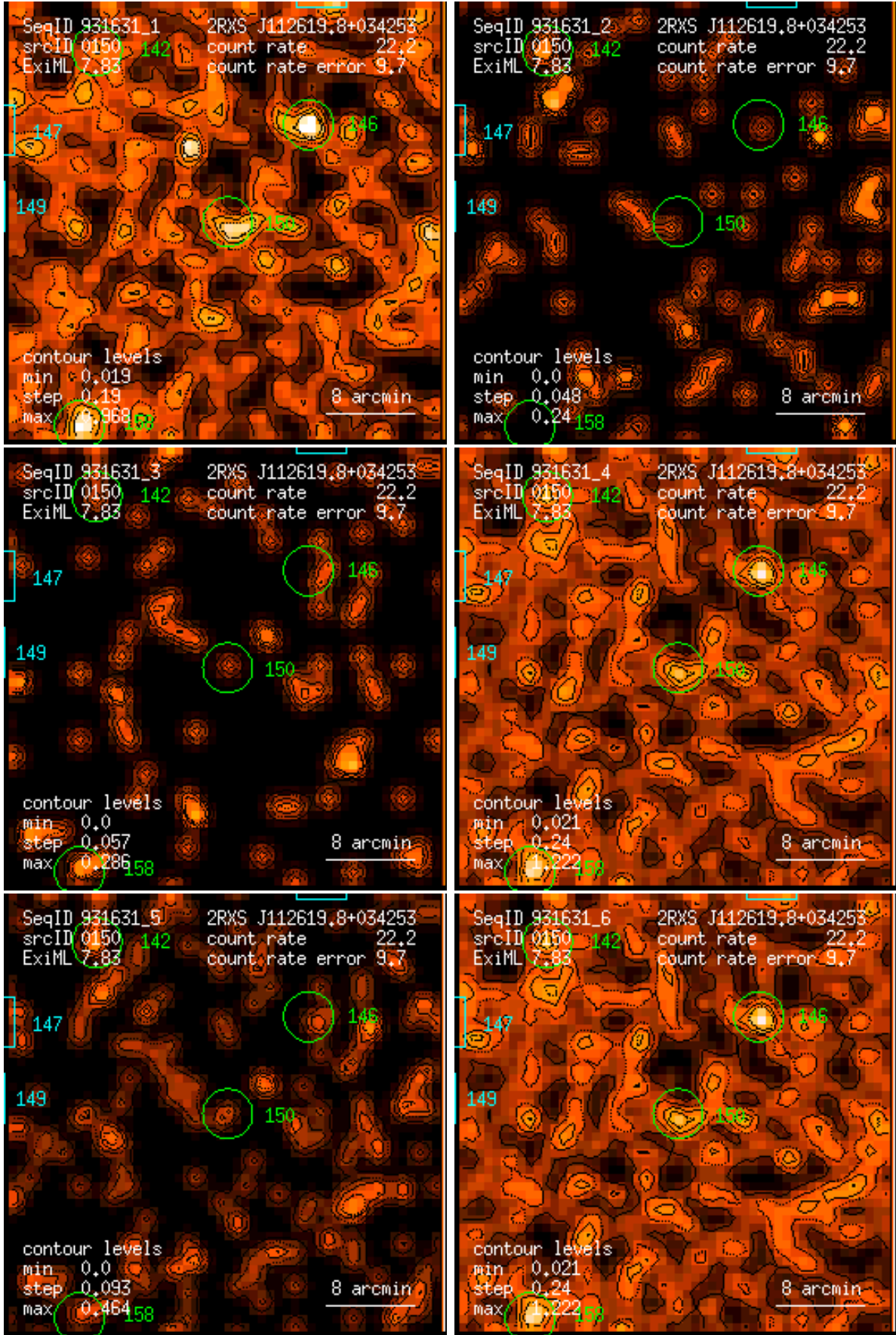
Figure 150: RASS 931631: detection 0150: band rate images, Gaussian filter: (1) PSPC channels 11 – 41, (2) 52 – 90, (3) 91 – 201, (4) 11 – 235, (5) 52 – 201, (6) 11 – 201. Broad band rates in counts/ks. Band rate contour levels in counts/ks/arcmin 2 .
