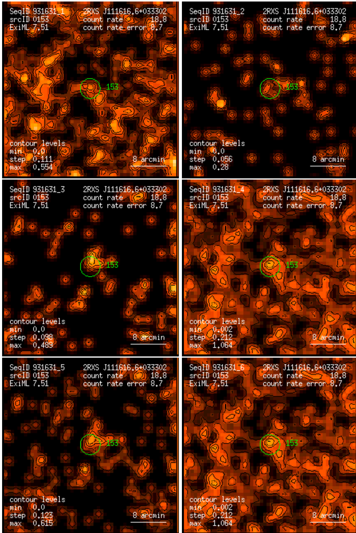
Figure 153: RASS 931631: detection 0153: band rate images, Gaussian filter: (1) PSPC channels 11 – 41, (2) 52 – 90, (3) 91 – 201, (4) 11 – 235, (5) 52 – 201, (6) 11 – 201. Broad band rates in counts/ks. Band rate contour levels in counts/ks/arcmin 2 .
